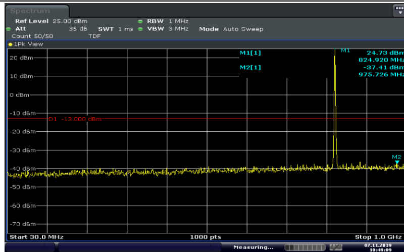
Band26-1.4MHz-QPSK-26797-6RB#0-Range3:30~1000MHz
