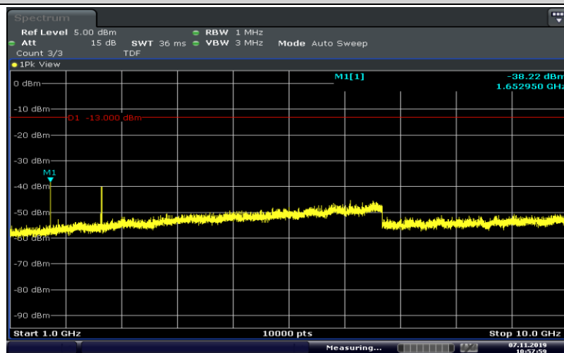
Band26-3MHz-QPSK-26805-15RB#0-Range4:1000~10000MHz
