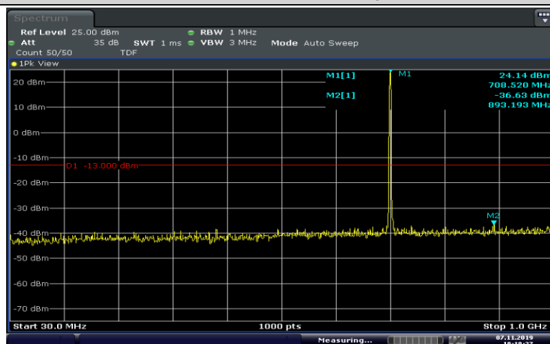
Band12-1.4MHz-QPSK-23095-6RB#0-Range1:30~1000MHz
