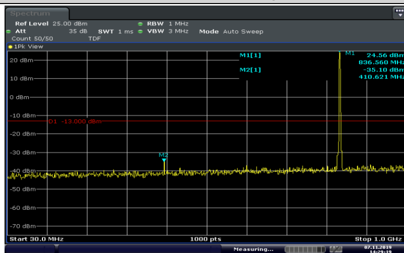
Band5-1.4MHz-QPSK-20525-6RB#0-Range3:30~1000MHz
