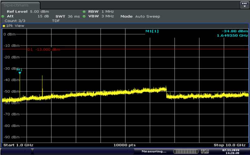
Band5-1.4MHz-16QAM-20407-6RB#0-Range4:1000~10000MHz
