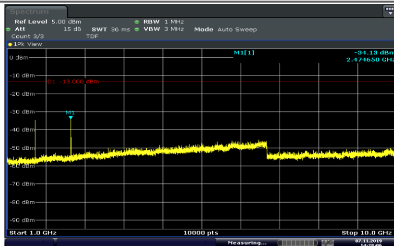
Band5-1.4MHz-QPSK-20407-6RB#0-Range4:1000~10000MHz
