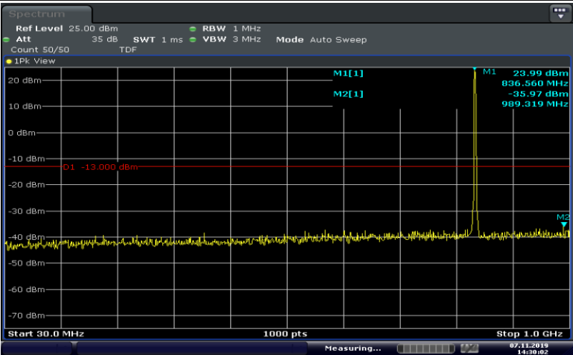
Band5-1.4MHz-16QAM-20525-6RB#0-Range3:30~1000MHz
