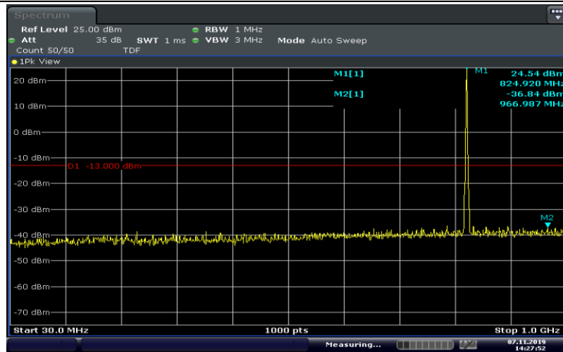
Band5-1.4MHz-QPSK-20407-6RB#0-Range3:30~1000MHz
