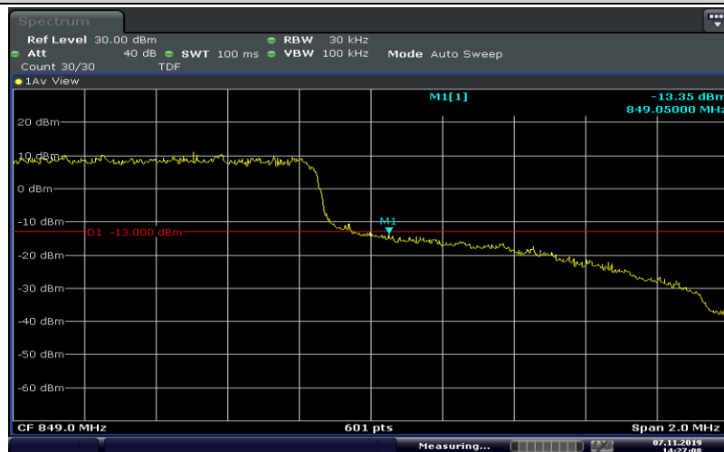
Band5-1.4MHz-QPSK-20643-6RB#0
