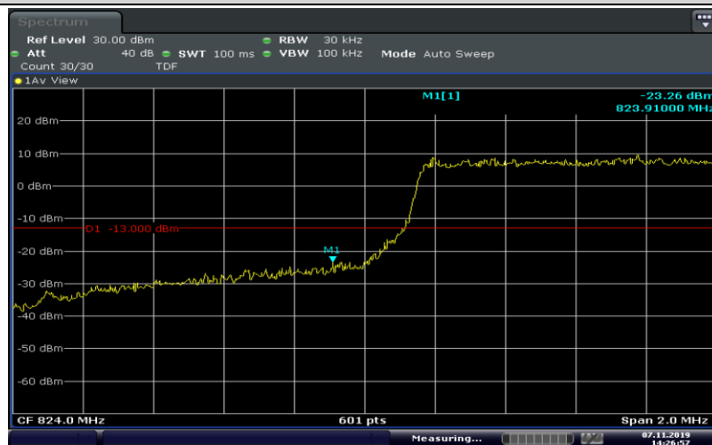
Band5-1.4MHz-16QAM-20407-6RB#0
