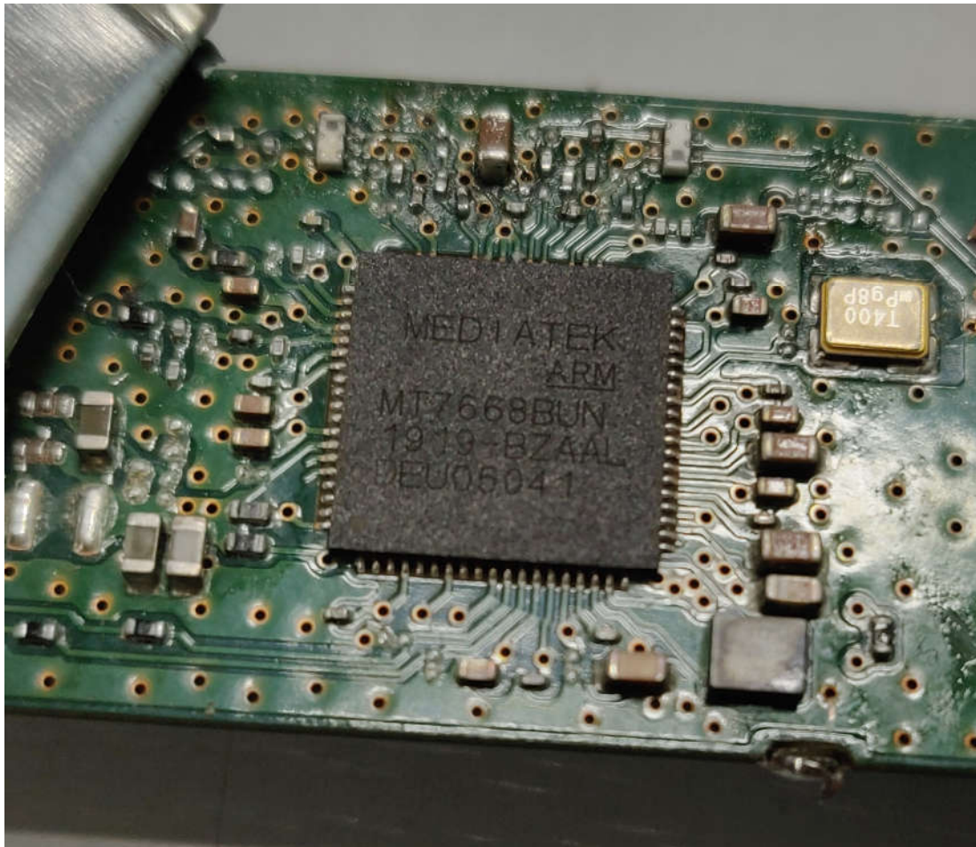
Figure 4 Inside of the EUT
