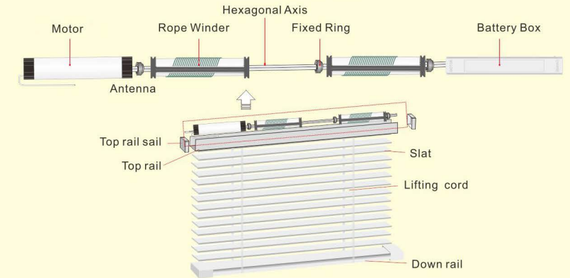
Diagram of the venetian blinds
