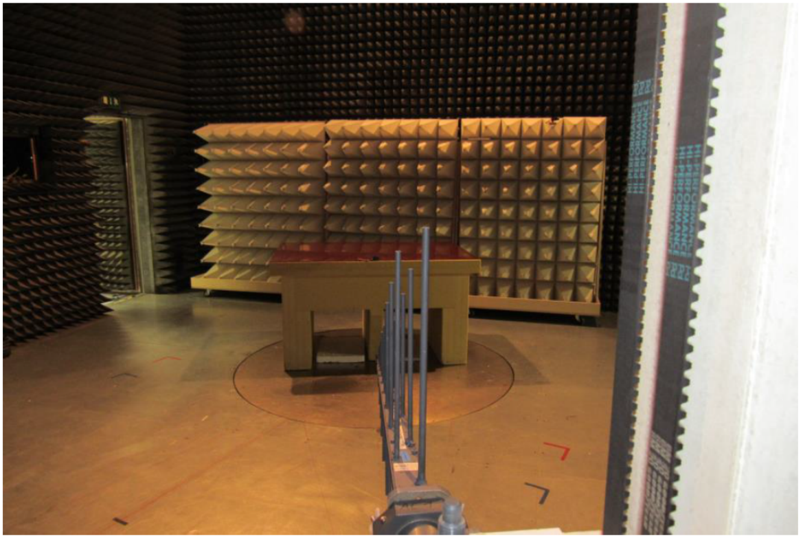
Testsetup view from antenna
