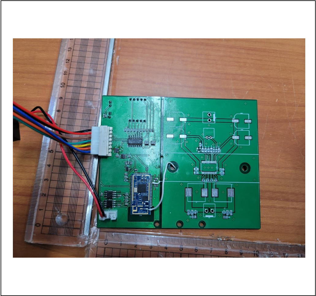
MainBoard-Rear
