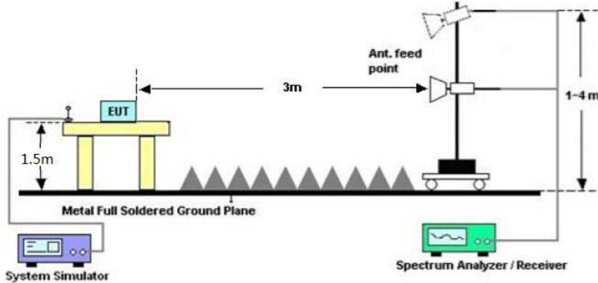
Radiated Emission Test-Setup Frequency Above 1000MHz
