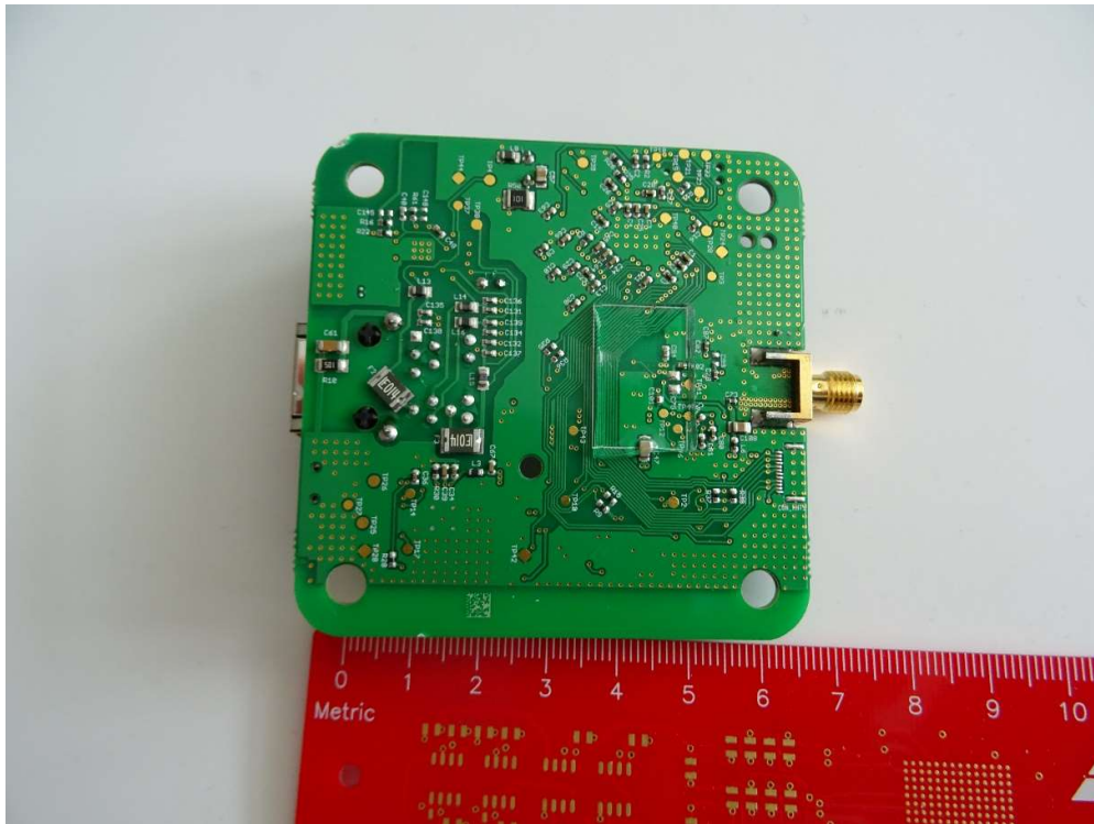
Photograph 3: bottom view
