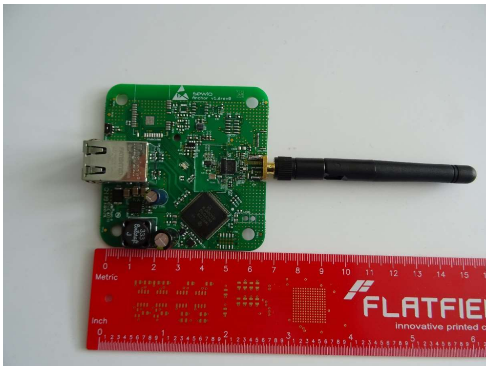
Photograph 1: top view with antenna
