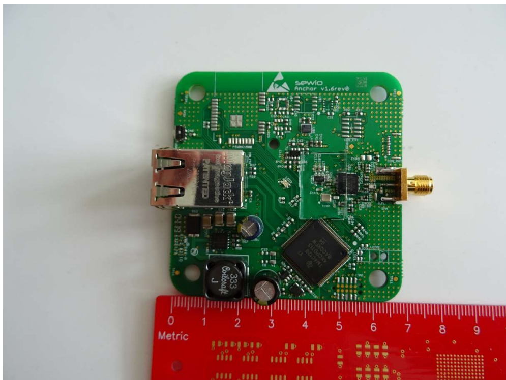
Photograph 2: : top view without antenna
