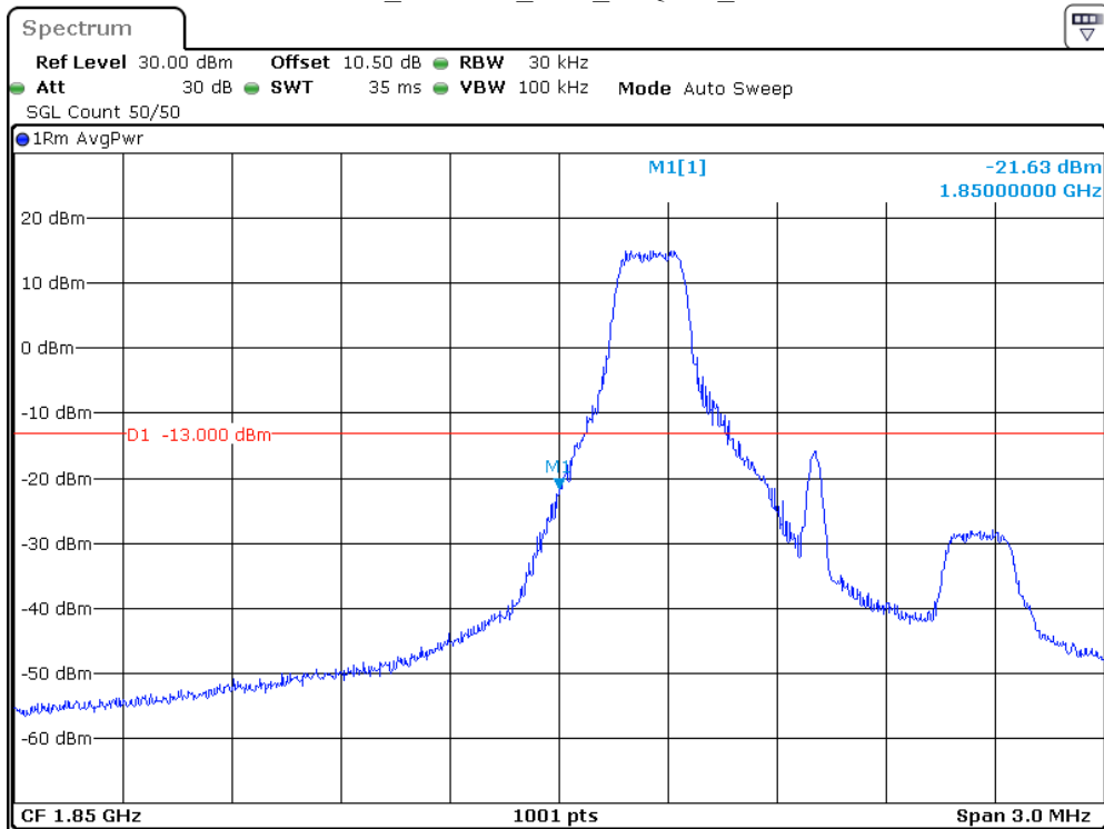
Band 2_1.4 MHz_Low_16QAM_RB1#0
