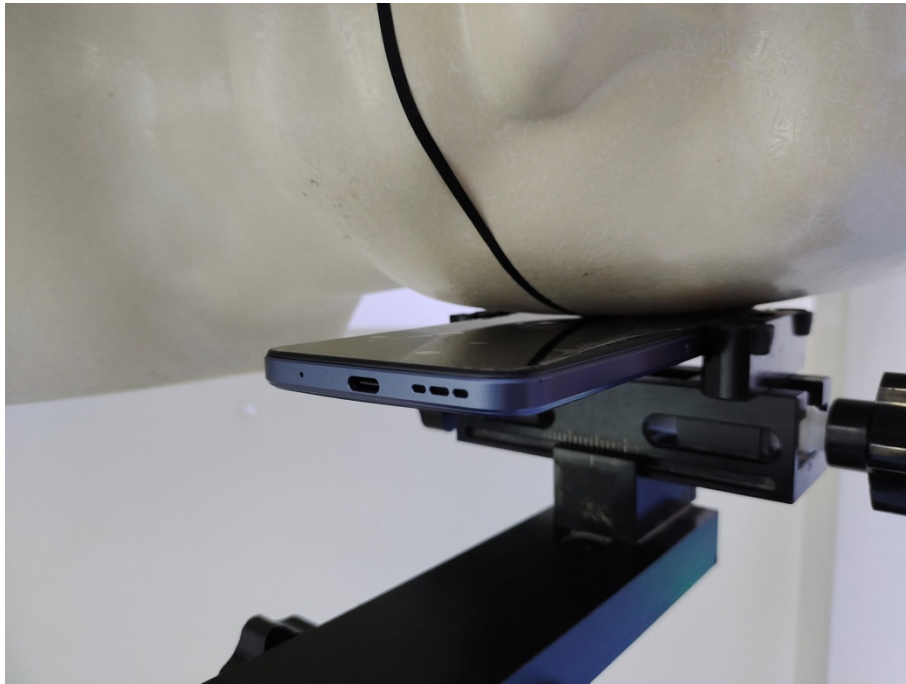
Head Left Check Setup Photo (0mm)
