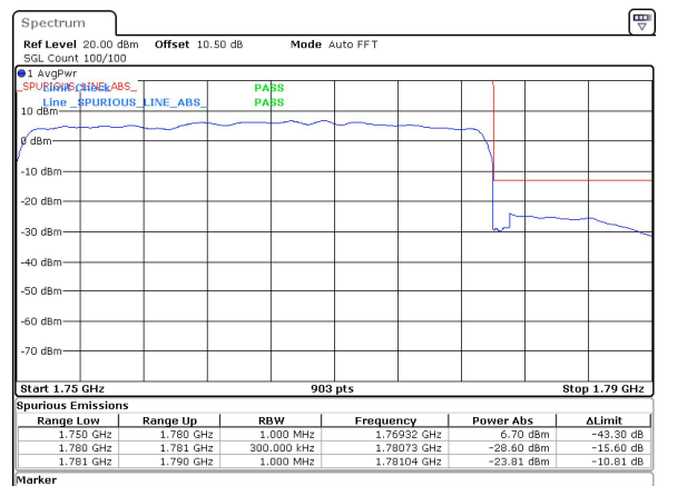
30MHz_15kHz_1765MHz_DFT-s-OFDM QPSK_RB160@0&-23.81 dBm
