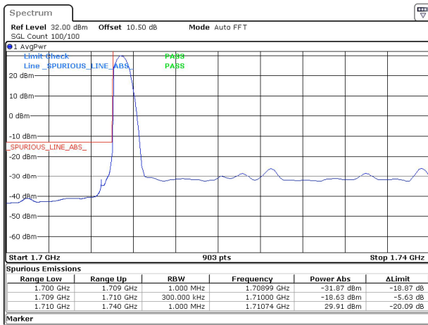
30MHz_15kHz_1725MHz_DFT-s-OFDM QPSK_RB1@0&-18.63 dBm
