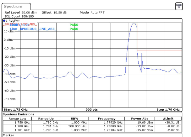
30MHz_15kHz_1765MHz_DFT-s-OFDM QPSK_RB1@159&-13.82 dBm
