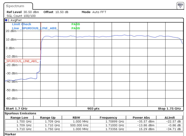
40MHz_15kHz_1730MHz_DFT-s-OFDM QPSK_RB216@0&-13.86 dBm
