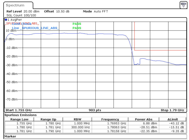
25MHz_15kHz_1767.5MHz_DFT-s-OFDM QPSK_RB128@0&-22.35 dBm
