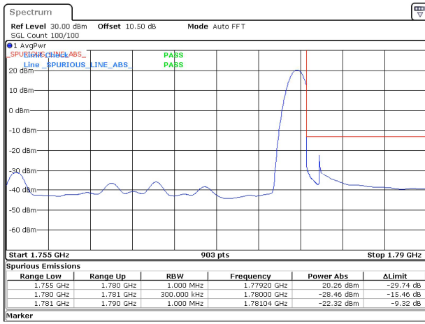
25MHz_15kHz_1767.5MHz_DFT-s-OFDM QPSK_RB1@132&-22.32 dBm
