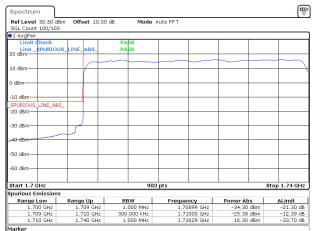
30MHz_15kHz_1725MHz_DFT-s-OFDM QPSK_RB160@0&-25.39 dBm
