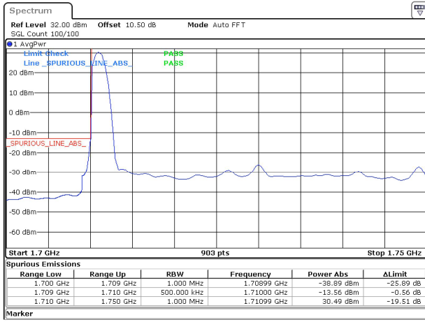
40MHz_15kHz_1730MHz_DFT-s-OFDM QPSK_RB1@0&-13.56 dBm
