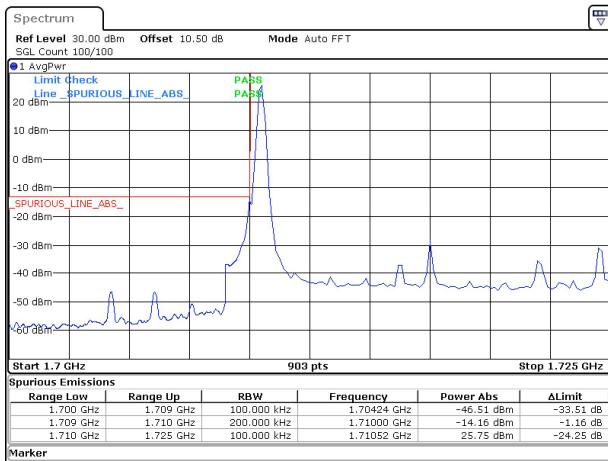
15MHz_15kHz_1717.5MHz_DFT-s-OFDM QPSK_RB1@0&-14.16 dBm
