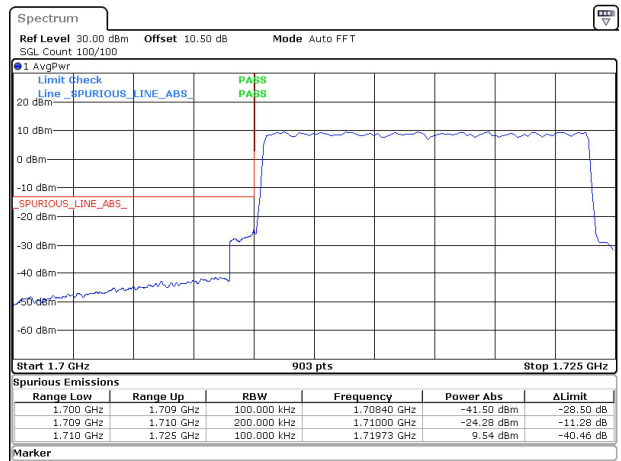
15MHz_15kHz_1717.5MHz_DFT-s-OFDM QPSK_RB75@0&-24.28 dBm
