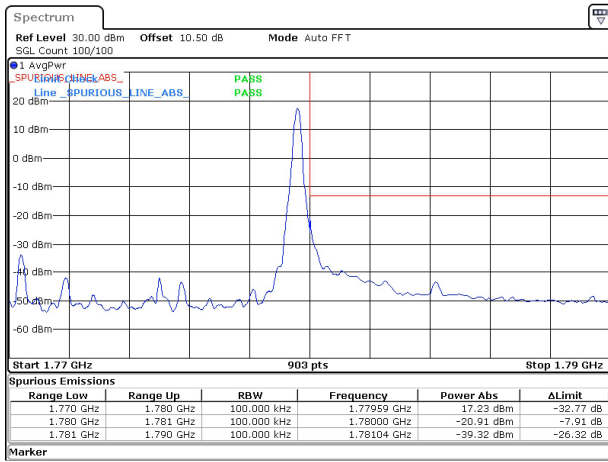
10MHz_15kHz_1775MHz_DFT-s-OFDM QPSK_RB1@51&-20.91 dBm
