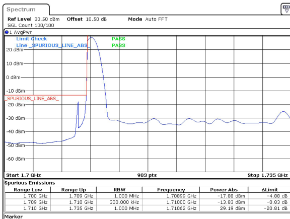
25MHz_15kHz_1722.5MHz_DFT-s-OFDM QPSK_RB1@0&-13.83 dBm
