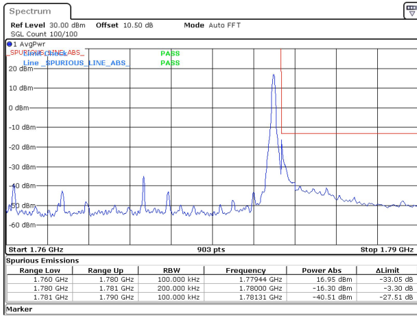
20MHz_15kHz_1770MHz_DFT-s-OFDM QPSK_RB1@105&-16.30 dBm
