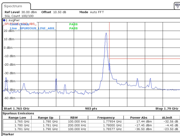
15MHz_15kHz_1772.5MHz_DFT-s-OFDM QPSK_RB1@78&-17.45 dBm
