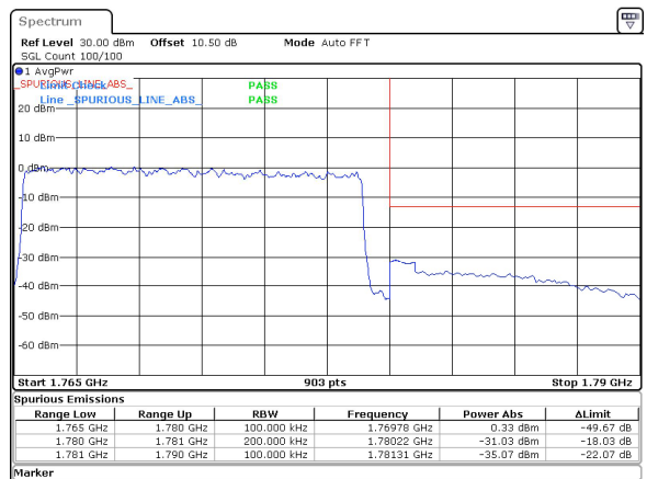
15MHz_15kHz_1772.5MHz_DFT-s-OFDM QPSK_RB75@0&-31.03 dBm
