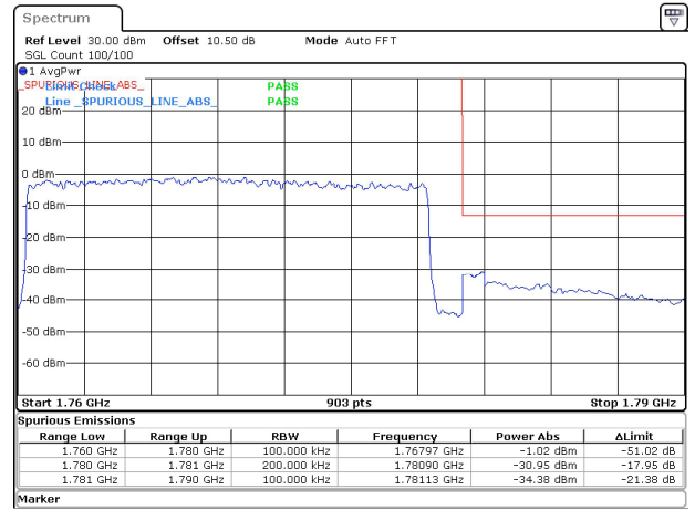
20MHz_15kHz_1770MHz_DFT-s-OFDM QPSK_RB100@0&-30.95 dBm
