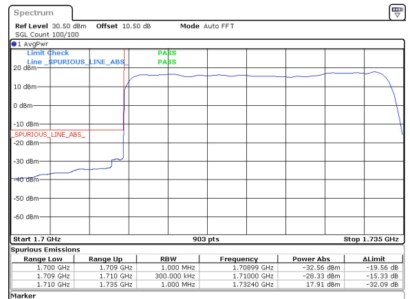
25MHz_15kHz_1722.5MHz_DFT-s-OFDM QPSK_RB128@0&-28.33 dBm
