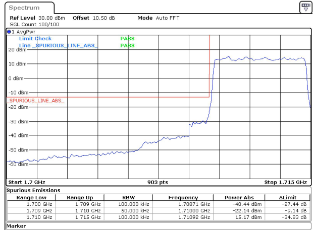
5MHz_15kHz_1712.5MHz_DFT-s-OFDM QPSK_RB25@0&-22.14 dBm
