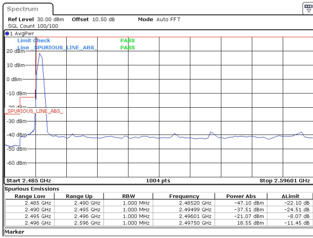
100MHz_30kHz_2546.01MHz_DFT-s-OFDM QPSK_RB1@0&-21.07 dBm
