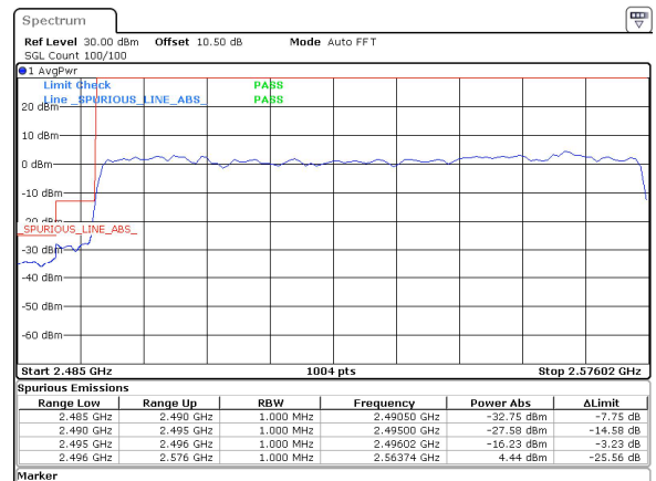
80MHz_30kHz_2536.02MHz_DFT-s-OFDM QPSK_RB216@0&-16.23 dBm
