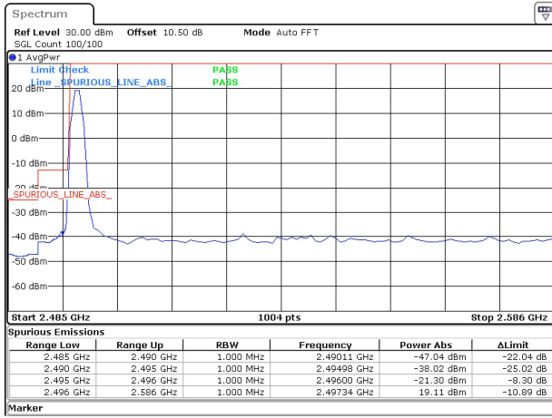
90MHz_30kHz_2541MHz_DFT-s-OFDM QPSK_RB1@0~-21.30 dBm
