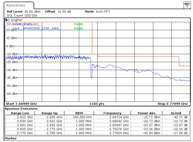
80MHz_30kHz_2649.99MHz_DFT-s-OFDM QPSK_RB216@0~-23.16 dBm
