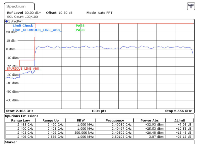
60MHz_30kHz_2526MHz_DFT-s-OFDM QPSK_RB162@0&-32.93 dBm
