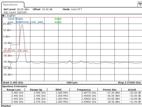
80MHz_30kHz_2536.02MHz_DFT-s-OFDM QPSK_RB1@0&-23.68 dBm
