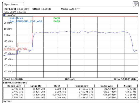
40MHz_30kHz_2516.01MHz_DFT-s-OFDM QPSK_RB100@0&-31.43 dBm
