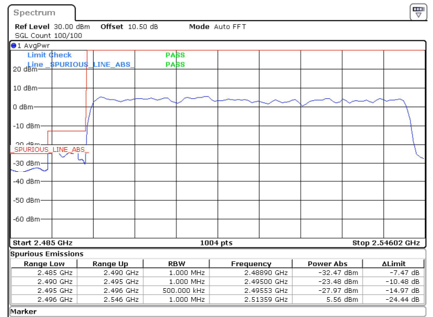
50MHz_30kHz_2521.02MHz_DFT-s-OFDM QPSK_RB128@0&-32.47 dBm
