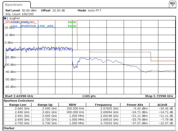
30MHz_30kHz_2674.98MHz_DFT-s-OFDM QPSK_RB75@0&-20.79 dBm
