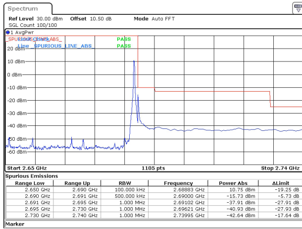
40MHz_30kHz_2670MHz_DFT-s-OFDM QPSK_RB1@105&-15.73 dBm
