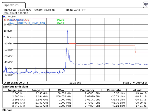
50MHz_30kHz_2664.99MHz_DFT-s-OFDM QPSK_RB1@132&-20.71 dBm
