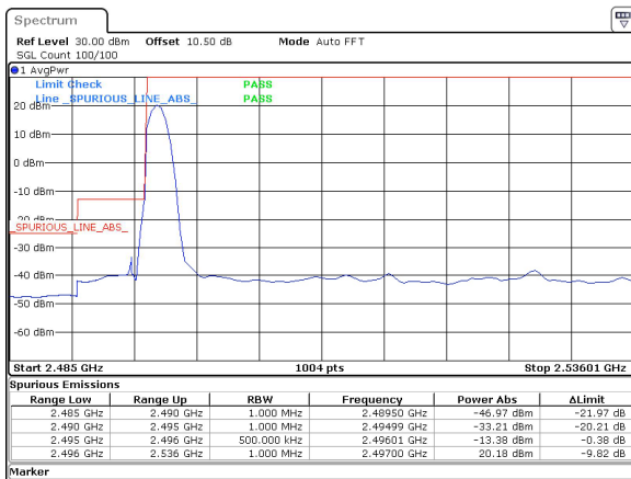
40MHz_30kHz_2516.01MHz_DFT-s-OFDM QPSK_RB1@0&-13.38 dBm
