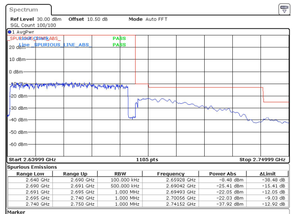
50MHz_30kHz_2664.99MHz_DFT-s-OFDM QPSK_RB128@0&-22.03 dBm
