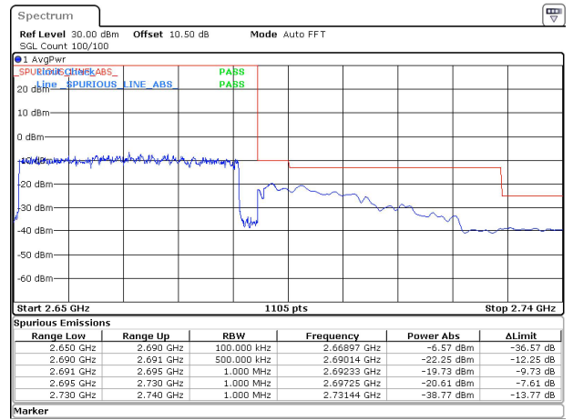
40MHz_30kHz_2670MHz_DFT-s-OFDM QPSK_RB100@0&-20.61 dBm
