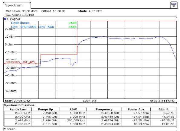
15MHz_30kHz_2503.5MHz_DFT-s-OFDM QPSK_RB36@0&-27.57 dBm
