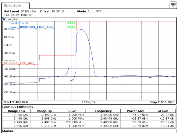
15MHz_30kHz_2503.5MHz_DFT-s-OFDM QPSK_RB1@0&19.79 dBm
