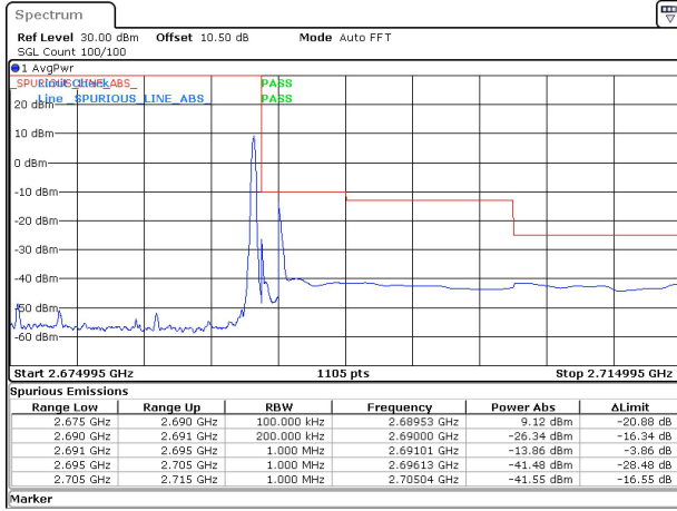
10MHz|15MHz_15kHz_1880MHz|2682.495MHz_DFT-s-OFDM QPSK_RB0|RB1@78&-13.86 dBm
