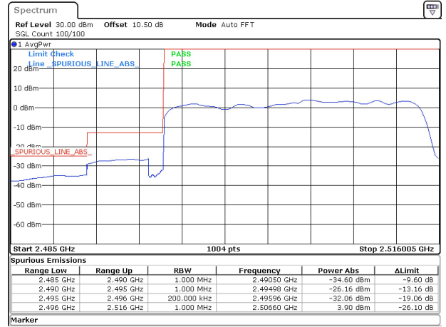
10MHz|20MHz_15kHz_1880MHz|2506.005MHz_DFT-s-OFDM QPSK_RB0|RB100@0&-34.60 dBm
