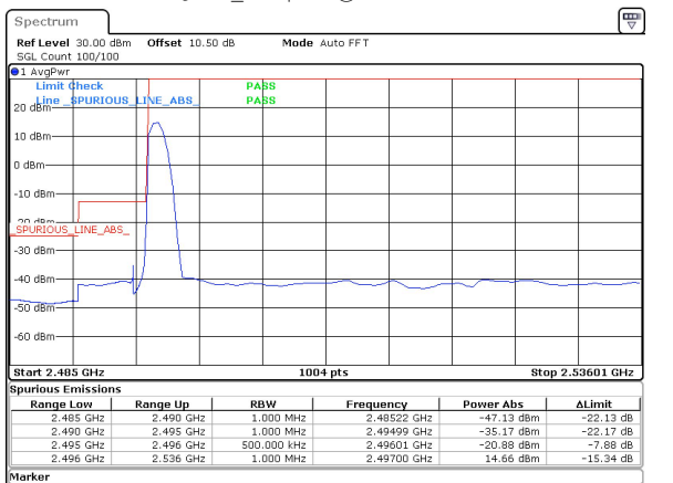
10MHz|40MHz 15kHz 1880MHz|2516.01MHz DFT-s-OFDM QPSK_RB0|RB1@0&-20.88 dBm
