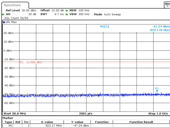
20MHz_15kHz_1720MHz_DFT-s-OFDM QPSK_RB1@105&-47.24 dBm
