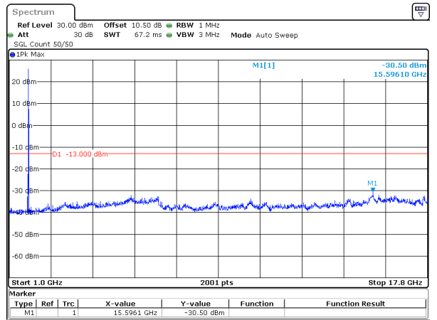
15MHz_15kHz_1772.5MHz_DFT-s-OFDM QPSK_RB1@78&-30.50 dBm
