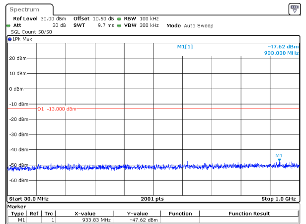
5MHz_15kHz_1777.5MHz_DFT-s-OFDM QPSK_RB1@24&-47.62 dBm
