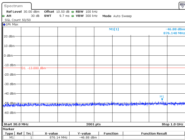
25MHz_15kHz_1722.5MHz_DFT-s-OFDM QPSK_RB128@0&-46.88 dBm
