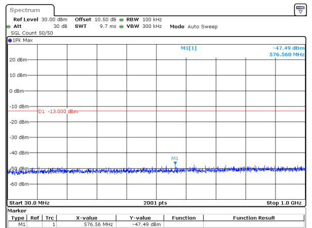
25MHz_15kHz_1745MHz_DFT-s-OFDM QPSK_RB128@0&-47.49 dBm
