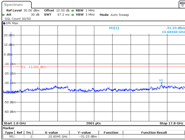
20MHz_15kHz_1745MHz_DFT-s-OFDM QPSK_RB1@105&-31.23 dBm
