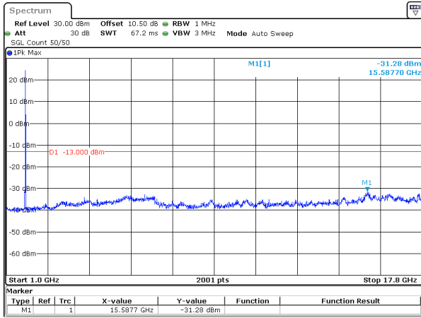
40MHz_15kHz_1760MHz_DFT-s-OFDM QPSK_RB1@215&-31.28 dBm
