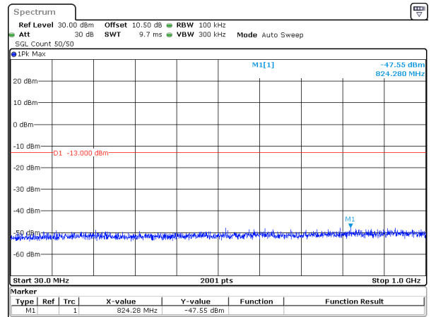
5MHz_15kHz_1745MHz_DFT-s-OFDM QPSK_RB1@24&-47.55 dBm
