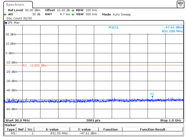
15MHz_15kHz_1745MHz_DFT-s-OFDM QPSK_RB1@0&-47.61 dBm
