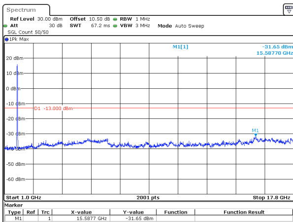
25MHz_15kHz_1745MHz_DFT-s-OFDM QPSK_RB128@0&-31.65 dBm
