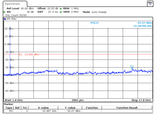
10MHz_15kHz_1715MHz_DFT-s-OFDM QPSK_RB1@0&-32.07 dBm
