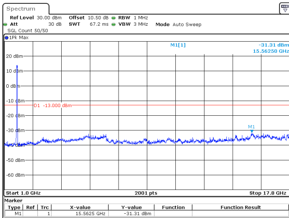
40MHz_15kHz_1745MHz_DFT-s-OFDM QPSK_RB216@0&-31.31 dBm
