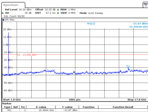
20MHz_15kHz_1720MHz_DFT-s-OFDM QPSK_RB100@0&-31.87 dBm
