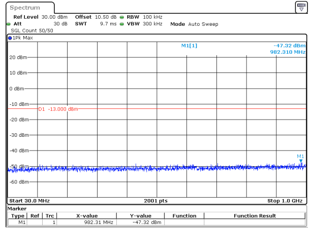
40MHz_15kHz_1760MHz_DFT-s-OFDM QPSK_RB1@215&-47.32 dBm
