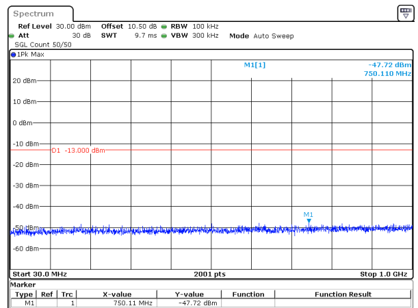
30MHz_15kHz_1725MHz_DFT-s-OFDM QPSK_RB160@0&-47.72 dBm
