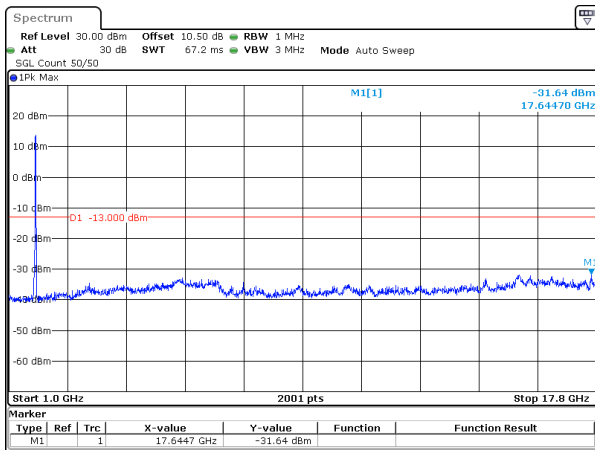
40MHz_15kHz_1760MHz_DFT-s-OFDM QPSK_RB216@0&-31.64 dBm
