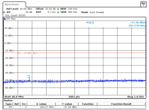
25MHz_15kHz_1767.5MHz_DFT-s-OFDM QPSK_RB1@0&-47.56 dBm
