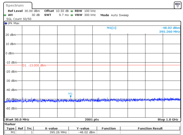
15MHz_15kHz_1745MHz_DFT-s-OFDM QPSK_RB75@0&-48.02 dBm
