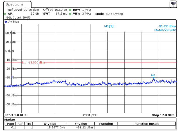
25MHz_15kHz_1722.5MHz_DFT-s-OFDM QPSK_RB1@0&-31.22 dBm
