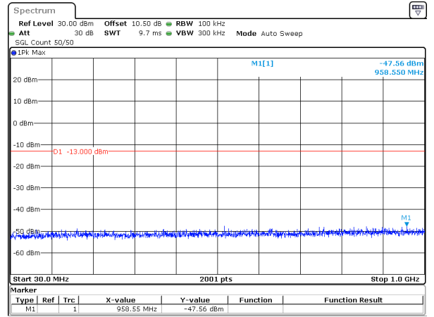
40MHz_15kHz_1745MHz_DFT-s-OFDM QPSK_RB1@215&-47.56 dBm
