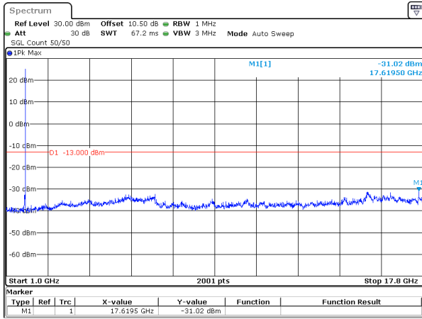
40MHz_15kHz_1745MHz_DFT-s-OFDM QPSK_RB1@215&-31.02 dBm
