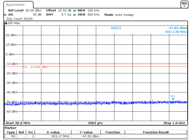
10MHz_15kHz_1775MHz_DFT-s-OFDM QPSK_RB1@0&-47.83 dBm
