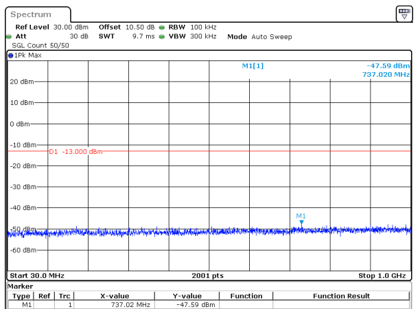
15MHz_15kHz_1717.5MHz_DFT-s-OFDM QPSK_RB75@0&-47.59 dBm
