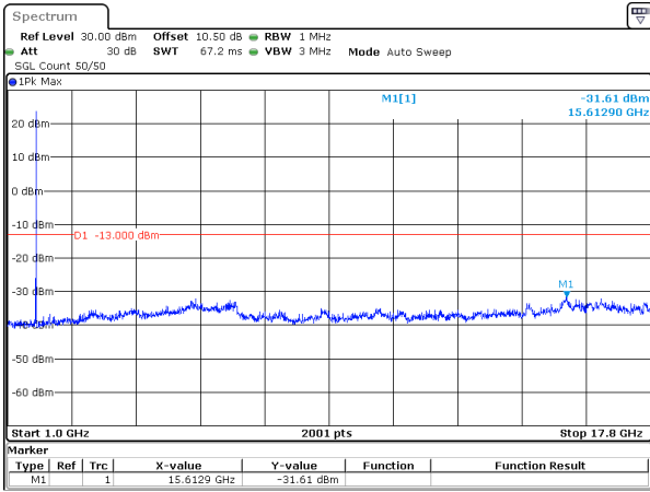
10MHz_15kHz_1745MHz_DFT-s-OFDM QPSK_RB1@51&-31.61 dBm
