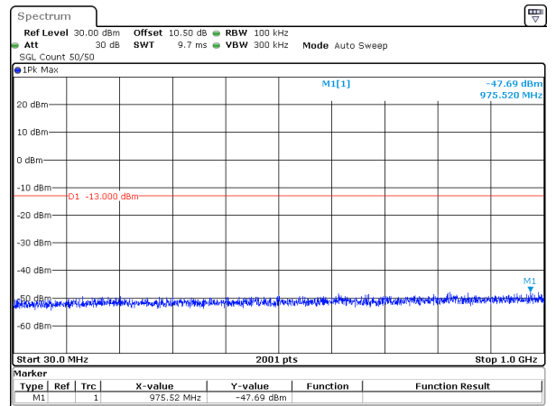
40MHz_15kHz_1745MHz_DFT-s-OFDM QPSK_RB216@0&-47.69 dBm
