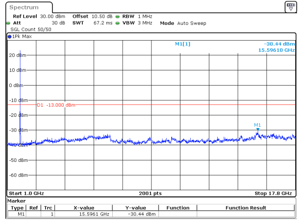
40MHz_15kHz_1760MHz_DFT-s-OFDM QPSK_RB1@0&-30.44 dBm
