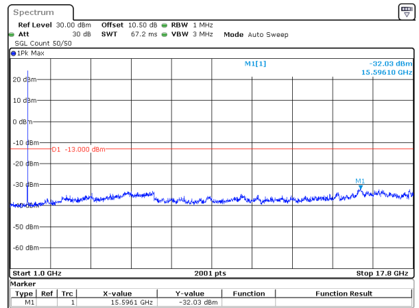
20MHz_15kHz_1720MHz_DFT-s-OFDM QPSK_RB1@105&-32.03 dBm
