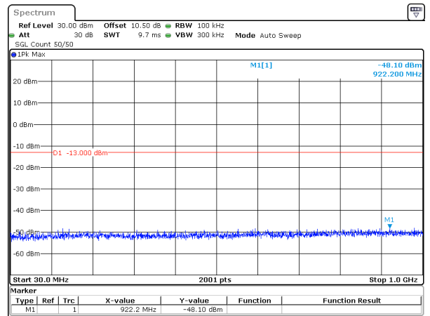
30MHz_15kHz_1745MHz_DFT-s-OFDM QPSK_RB160@0&-48.10 dBm
