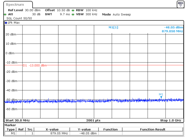
20MHz_15kHz_1745MHz_DFT-s-OFDM QPSK_RB1@0&-48.05 dBm
