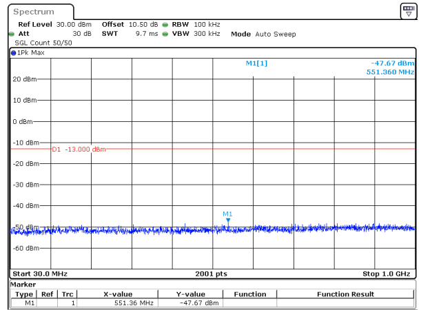
30MHz_15kHz_1725MHz_DFT-s-OFDM QPSK_RB1@0&-47.67 dBm
