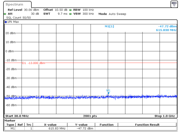
40MHz_15kHz_1730MHz_DFT-s-OFDM QPSK_RB1@0&-47.72 dBm
