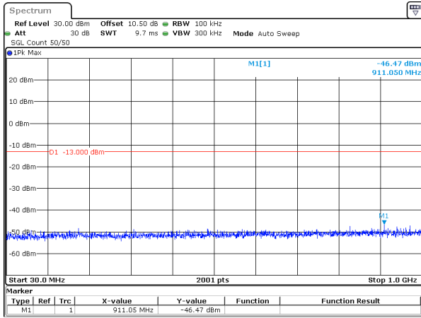
20MHz_15kHz_1770MHz_DFT-s-OFDM QPSK_RB1@105&-46.47 dBm
