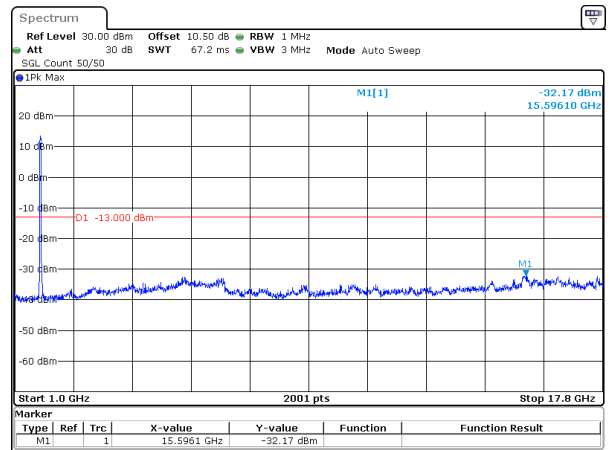
40MHz_15kHz_1730MHz_DFT-s-OFDM QPSK_RB216@0&-32.17 dBm
