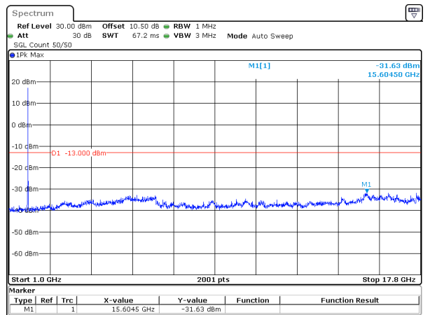
15MHz_15kHz_1772.5MHz_DFT-s-OFDM QPSK_RB75@0&-31.63 dBm
