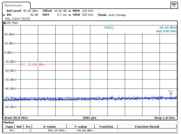
15MHz_15kHz_1717.5MHz_DFT-s-OFDM QPSK_RB1@0&-46.68 dBm
