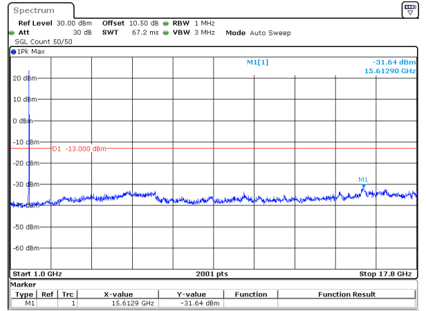
30MHz_15kHz_1765MHz_DFT-s-OFDM QPSK_RB1@159&-31.64 dBm
