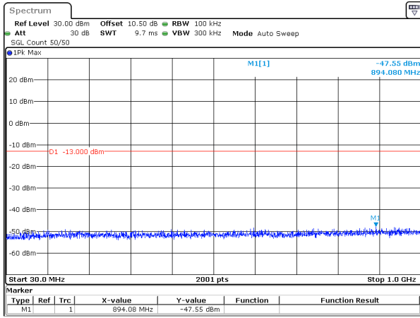
25MHz_15kHz_1722.5MHz_DFT-s-OFDM QPSK_RB1@0&-47.55 dBm
