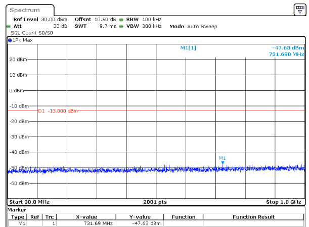
20MHz_15kHz_1720MHz_DFT-s-OFDM QPSK_RB100@0&-47.63 dBm
