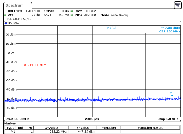
30MHz_15kHz_1725MHz_DFT-s-OFDM QPSK_RB1@159&-47.55 dBm
