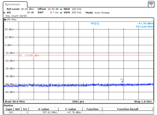
25MHz_15kHz_1722.5MHz_DFT-s-OFDM QPSK_RB1@132&-47.76 dBm
