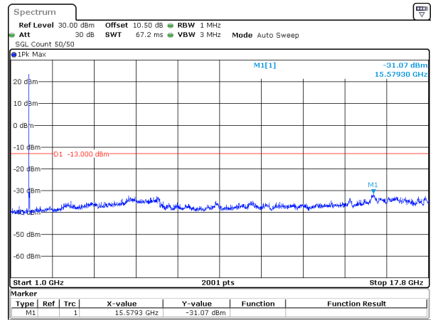
25MHz_15kHz_1745MHz_DFT-s-OFDM QPSK_RB1@0&-31.07 dBm
