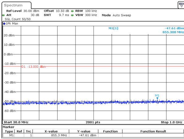
30MHz_15kHz_1765MHz_DFT-s-OFDM QPSK_RB1@0&-47.61 dBm
