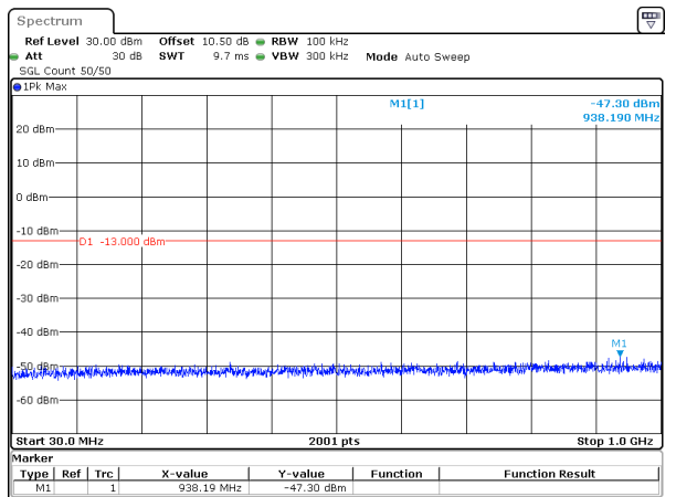
15MHz_15kHz_1717.5MHz_DFT-s-OFDM QPSK_RB1@78&-47.30 dBm
