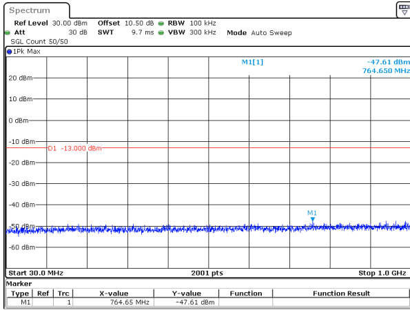
30MHz_15kHz_1765MHz_DFT-s-OFDM QPSK_RB1@159&-47.61 dBm
