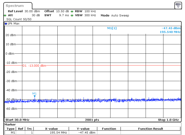
25MHz_15kHz_1767.5MHz_DFT-s-OFDM QPSK_RB128@0&-47.45 dBm
