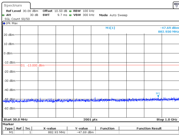
20MHz_15kHz_1745MHz_DFT-s-OFDM QPSK_RB100@0&-47.69 dBm
