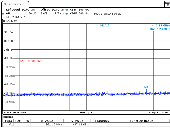
40MHz_15kHz_1760MHz_DFT-s-OFDM QPSK_RB1@0&-47.14 dBm
