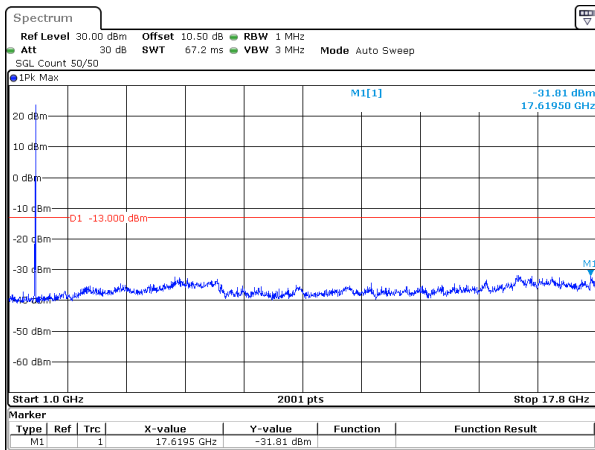
25MHz_15kHz_1745MHz_DFT-s-OFDM QPSK_RB1@132&-31.81 dBm
