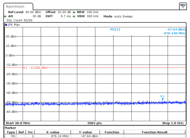
5MHz_15kHz_1777.5MHz_DFT-s-OFDM QPSK_RB25@0&-47.64 dBm
