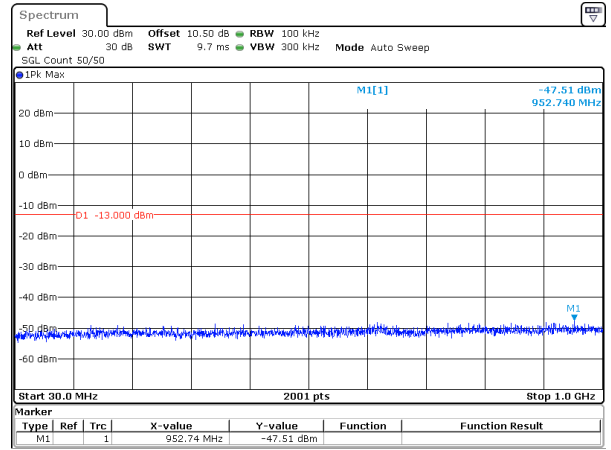
15MHz_15kHz_1745MHz_DFT-s-OFDM QPSK_RB1@78&-47.51 dBm
