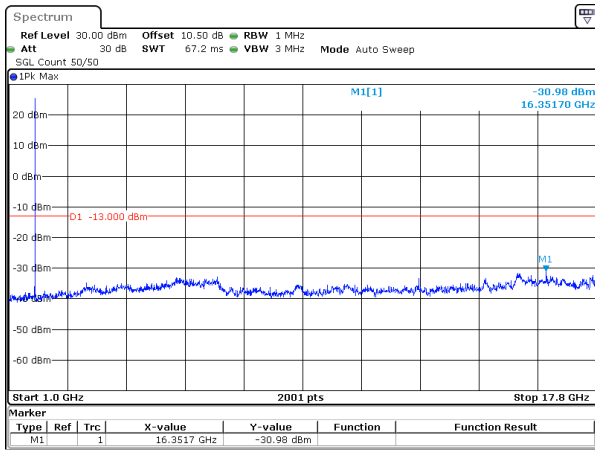
5MHz_15kHz_1745MHz_DFT-s-OFDM QPSK_RB1@0&-30.98 dBm
