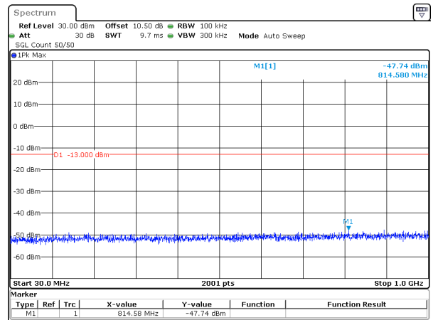
30MHz_15kHz_1765MHz_DFT-s-OFDM QPSK_RB160@0&-47.74 dBm
