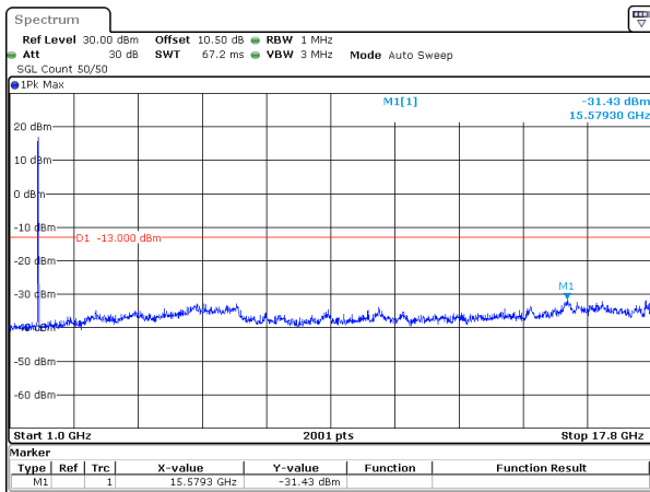
15MHz_15kHz_1745MHz_DFT-s-OFDM QPSK_RB75@0&-31.43 dBm
