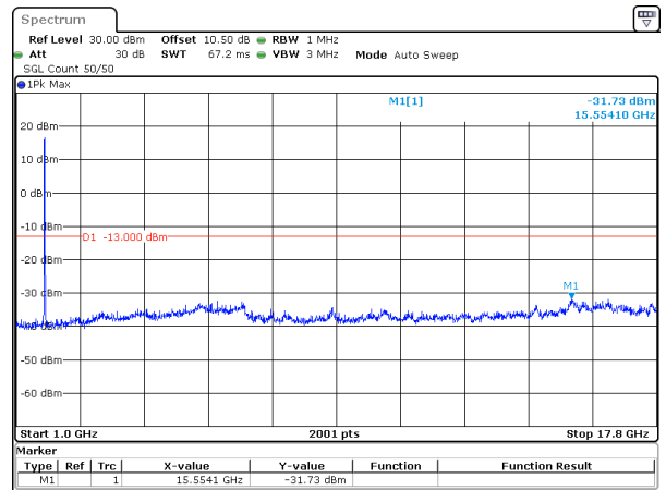
20MHz_15kHz_1745MHz_DFT-s-OFDM QPSK_RB100@0&-31.73 dBm
