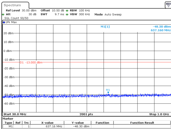
40MHz_15kHz_1730MHz_DFT-s-OFDM QPSK_RB216@0&-48.30 dBm
