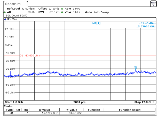
20MHz_15kHz_1770MHz_DFT-s-OFDM QPSK_RB1@105&-31.45 dBm
