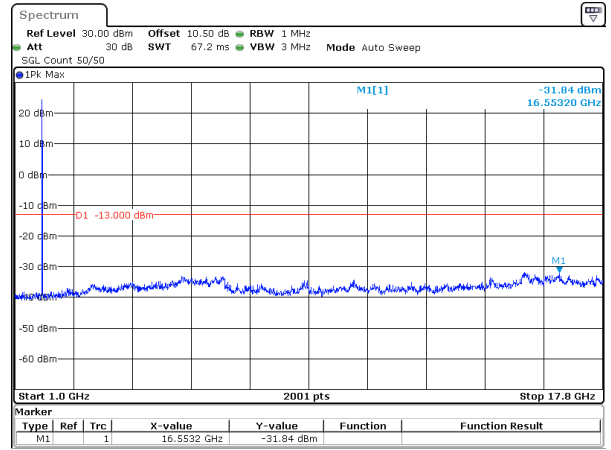
10MHz_15kHz_1775MHz_DFT-s-OFDM QPSK_RB1@51&-31.84 dBm
