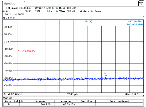
10MHz_15kHz_1745MHz_DFT-s-OFDM QPSK_RB1@51&-47.59 dBm
