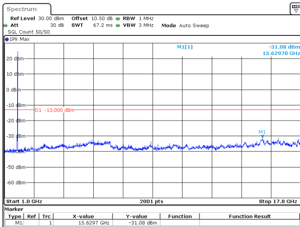
30MHz_15kHz_1725MHz_DFT-s-OFDM QPSK_RB1@159&-31.08 dBm
