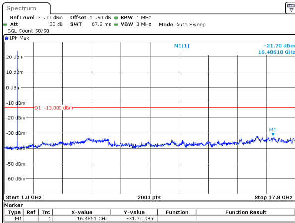
5MHz_15kHz_1745MHz_DFT-s-OFDM QPSK_RB1@24&-31.70 dBm
