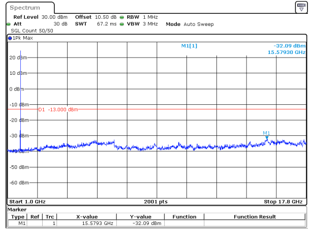
10MHz_15kHz_1715MHz_DFT-s-OFDM QPSK_RB1@51&-32.09 dBm
