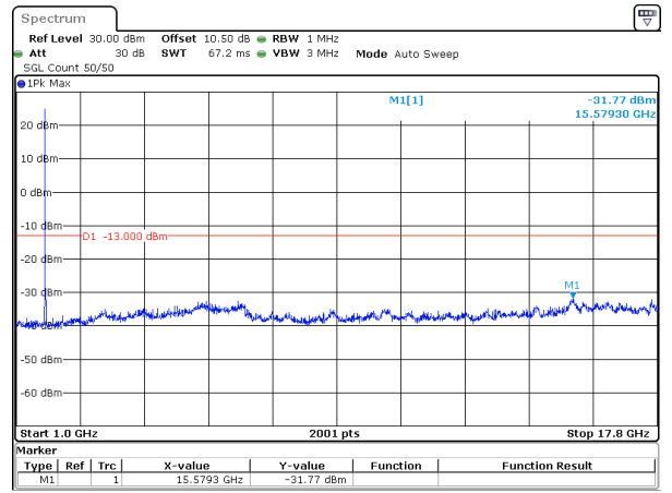
30MHz_15kHz_1765MHz_DFT-s-OFDM QPSK_RB1@0&-31.77 dBm
