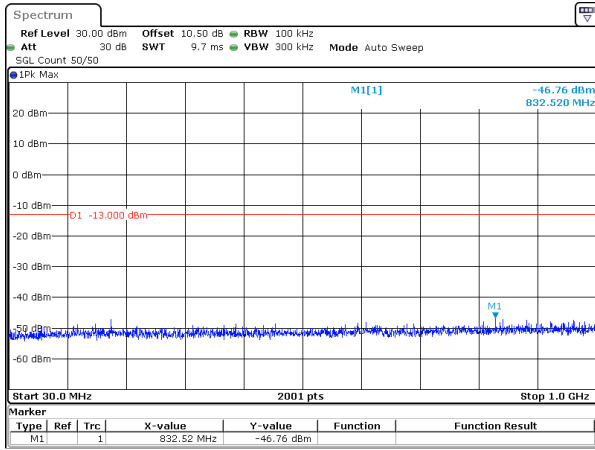
10MHz_15kHz_1715MHz_DFT-s-OFDM QPSK_RB1@51&-46.76 dBm
