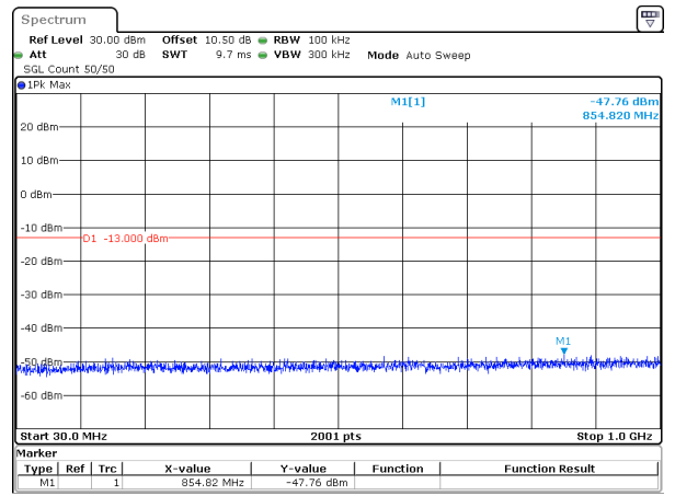
5MHz_15kHz_1777.5MHz_DFT-s-OFDM QPSK_RB1@0&-47.76 dBm
