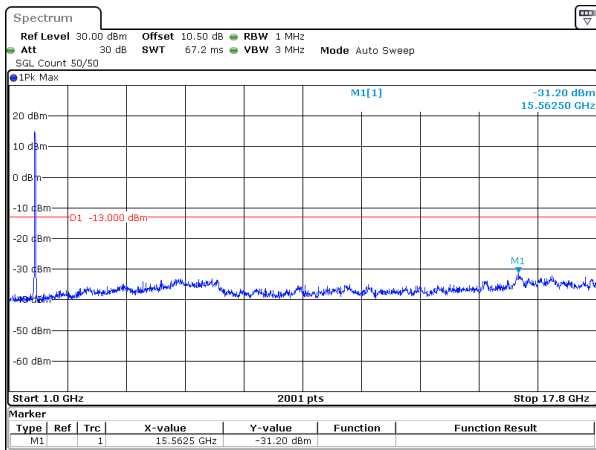
30MHz_15kHz_1745MHz_DFT-s-OFDM QPSK_RB160@0&-31.20 dBm
