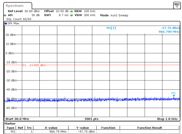
5MHz_15kHz_1745MHz_DFT-s-OFDM QPSK_RB25@0&-47.75 dBm
