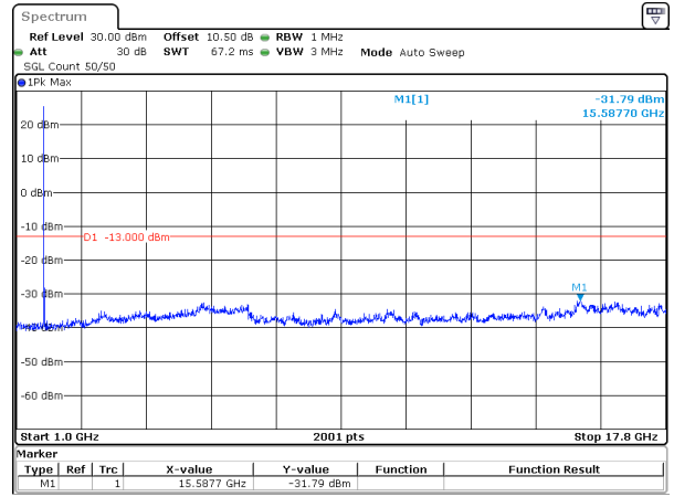
5MHz_15kHz_1712.5MHz_DFT-s-OFDM QPSK_RB1@0&-31.79 dBm
