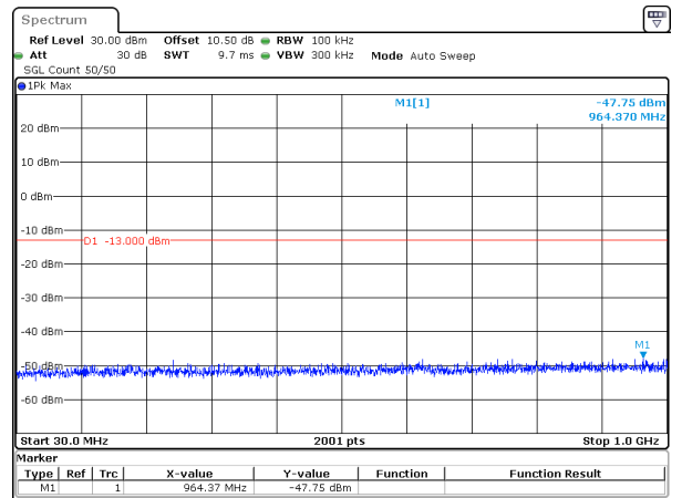
40MHz_15kHz_1760MHz_DFT-s-OFDM QPSK_RB216@0&-47.75 dBm
