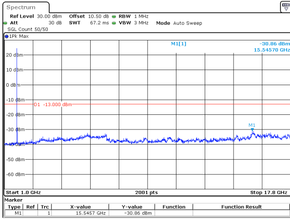
20MHz_15kHz_1745MHz_DFT-s-OFDM QPSK_RB1@0&-30.86 dBm
