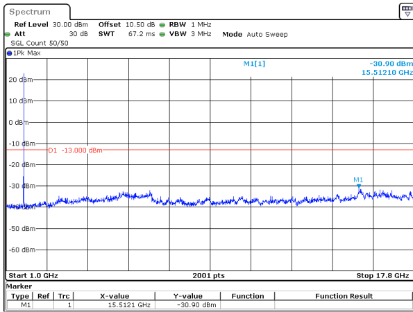
25MHz_15kHz_1722.5MHz_DFT-s-OFDM QPSK_RB1@132&-30.90 dBm
