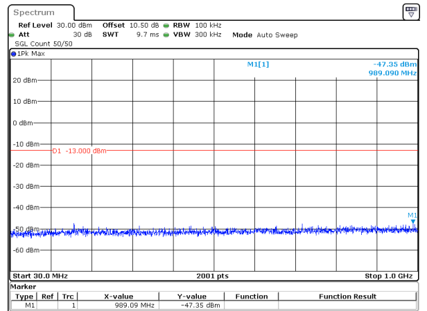
25MHz_15kHz_1745MHz_DFT-s-OFDM QPSK_RB1@132&-47.35 dBm
