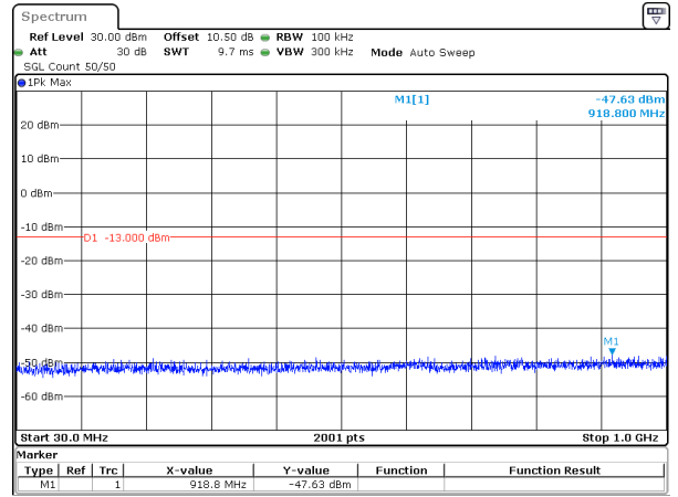
30MHz_15kHz_1745MHz_DFT-s-OFDM QPSK_RB1@159&-47.63 dBm
