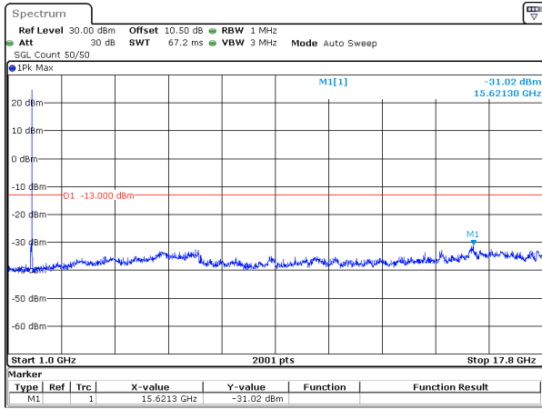
40MHz_15kHz_1730MHz_DFT-s-OFDM QPSK_RB1@215&-31.02 dBm
