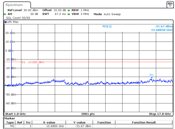
5MHz_15kHz_1712.5MHz_DFT-s-OFDM QPSK_RB1@24&-31.67 dBm
