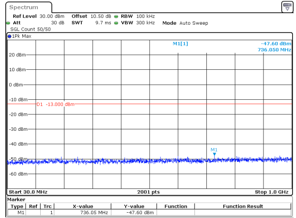
20MHz_15kHz_1745MHz_DFT-s-OFDM QPSK_RB1@105&-47.60 dBm
