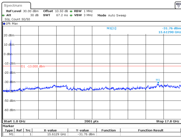
30MHz_15kHz_1765MHz_DFT-s-OFDM QPSK_RB160@0&-31.76 dBm
