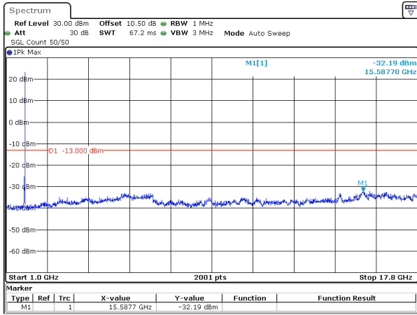
30MHz_15kHz_1745MHz_DFT-s-OFDM QPSK_RB1@159&-32.19 dBm
