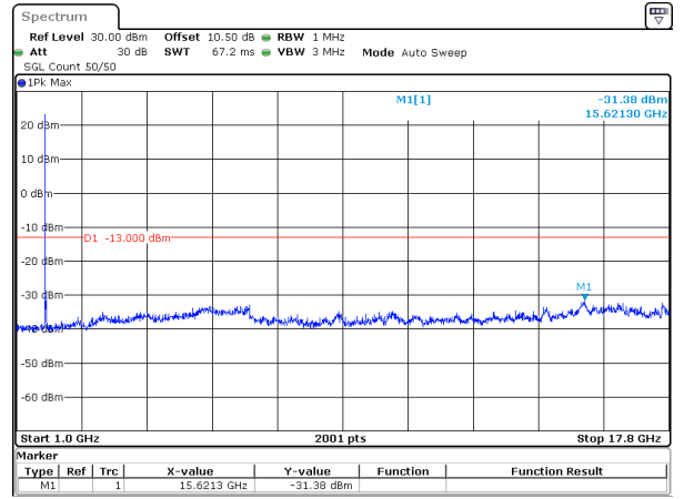
40MHz_15kHz_1745MHz_DFT-s-OFDM QPSK_RB1@0&-31.38 dBm
