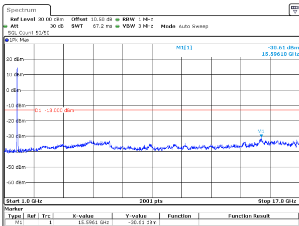
30MHz_15kHz_1725MHz_DFT-s-OFDM QPSK_RB160@0&-30.61 dBm
