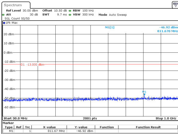
25MHz_15kHz_1745MHz_DFT-s-OFDM QPSK_RB1@0&-46.92 dBm
