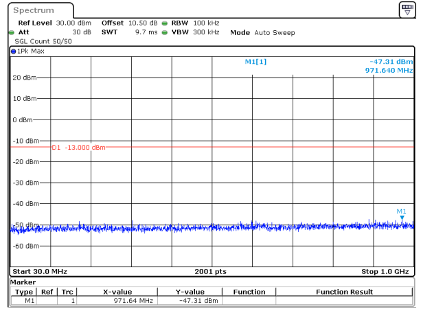
30MHz_15kHz_1745MHz_DFT-s-OFDM QPSK_RB1@0&-47.31 dBm
