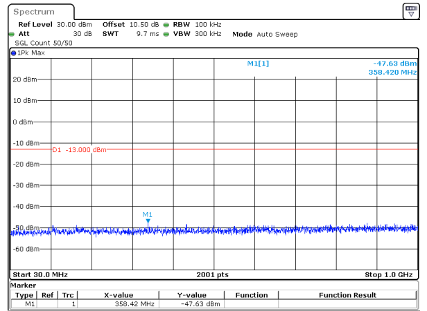
25MHz_15kHz_1767.5MHz_DFT-s-OFDM QPSK_RB1@132&-47.63 dBm
