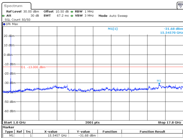
5MHz_15kHz_1745MHz_DFT-s-OFDM QPSK_RB25@0&-31.68 dBm
