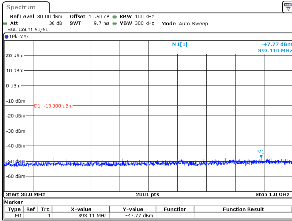
10MHz_15kHz_1775MHz_DFT-s-OFDM QPSK_RB1@51&-47.77 dBm
