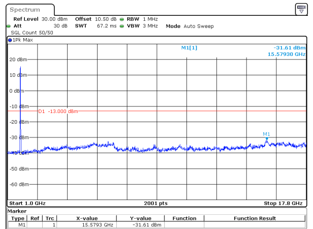
25MHz_15kHz_1722.5MHz_DFT-s-OFDM QPSK_RB128@0&-31.61 dBm
