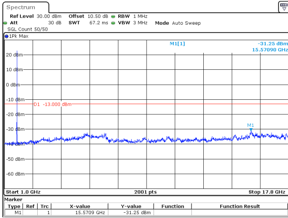
15MHz_15kHz_1745MHz_DFT-s-OFDM QPSK_RB1@78&-31.25 dBm
