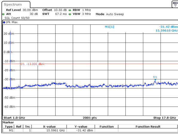
30MHz_15kHz_1745MHz_DFT-s-OFDM QPSK_RB1@0&-31.42 dBm
