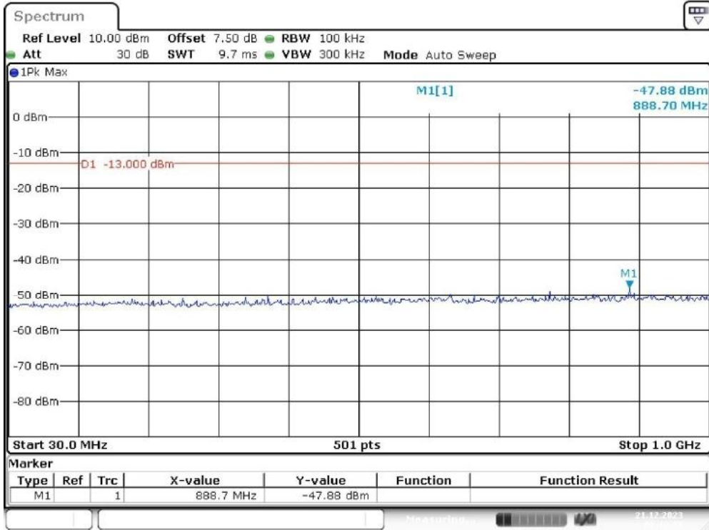
Band 2_1.4 MHz_Low_QPSK_RB6#0_1(30MHz-1GHz)
