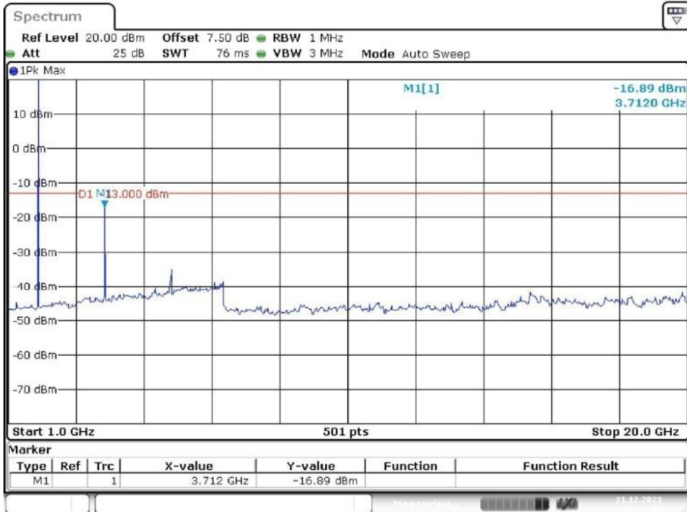
Band 2_1.4 MHz_Low_QPSK_RB6#0_2(1GHz-20GHz)
