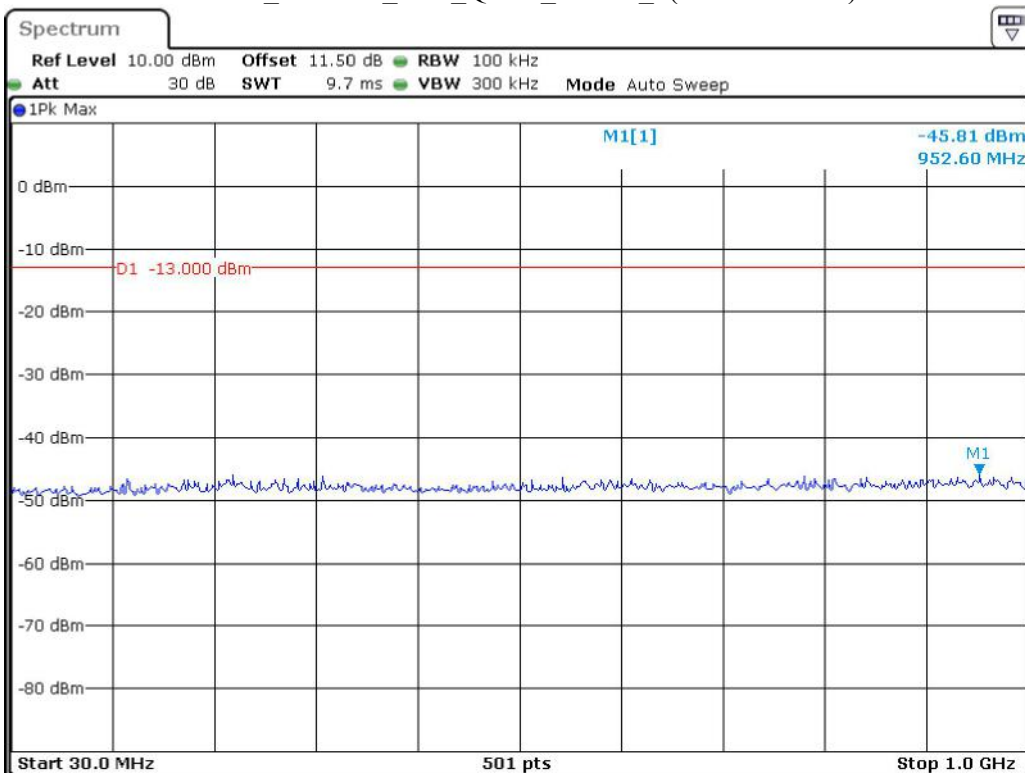
Band 2_1.4 MHz_Low_QPSK_RB6#0_1(30MHz-1GHz)
