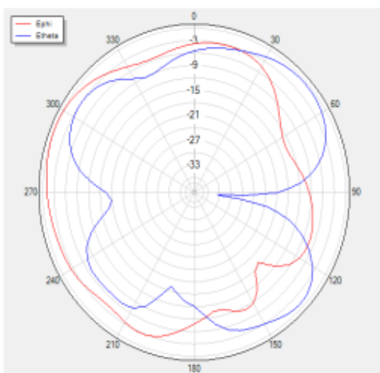
V Phi=90 freq=1720MHz
