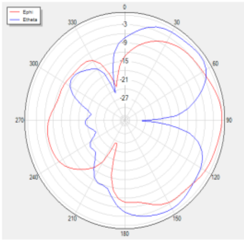
V Phi=90 freq=900MHz
