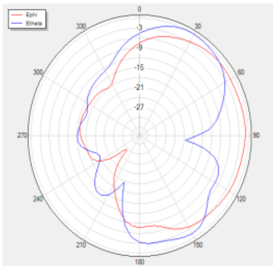
V Phi=90 freq=820MHz
