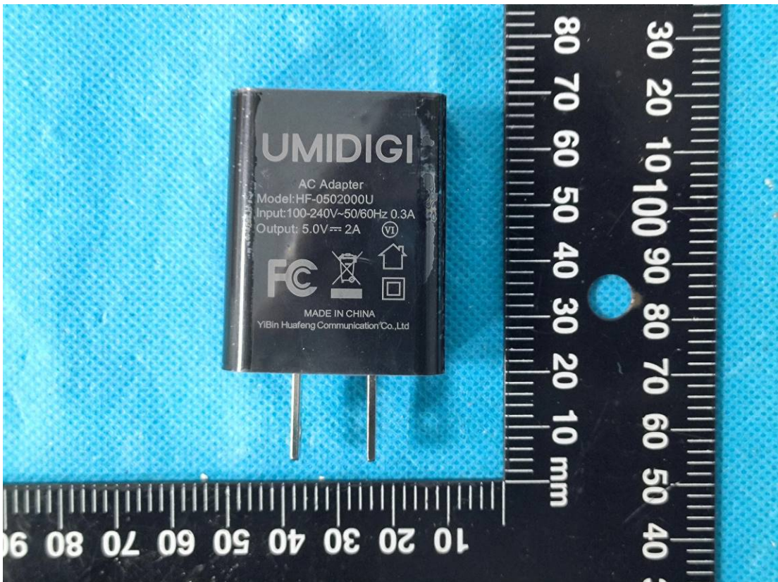
Adapter 1#
