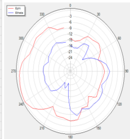
H Theta=90 freq=5800MHz
