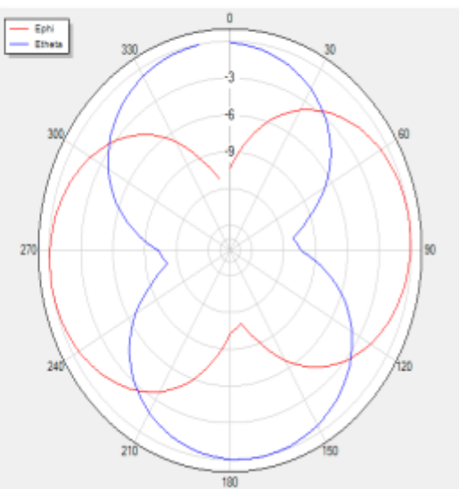
H Theta=0 freq=5400MHz
