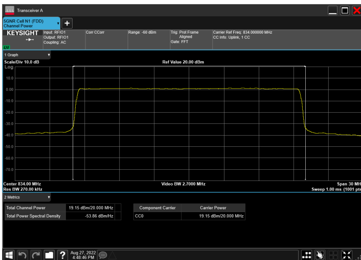
n5_20MHz_15kHz_834MHz_CP-OFDM 64 QAM_RB106@0
