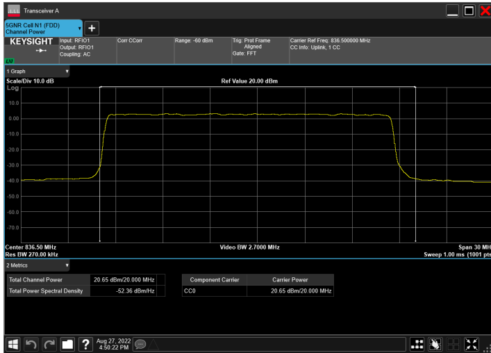
n5_20MHz_15kHz_836.5MHz_DFT-s-OFDM 16 QAM_RB100@0
