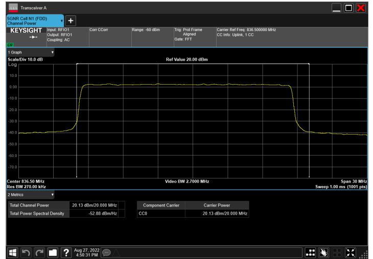
n5_20MHz_15kHz_836.5MHz_DFT-s-OFDM 64 QAM_RB100@0
