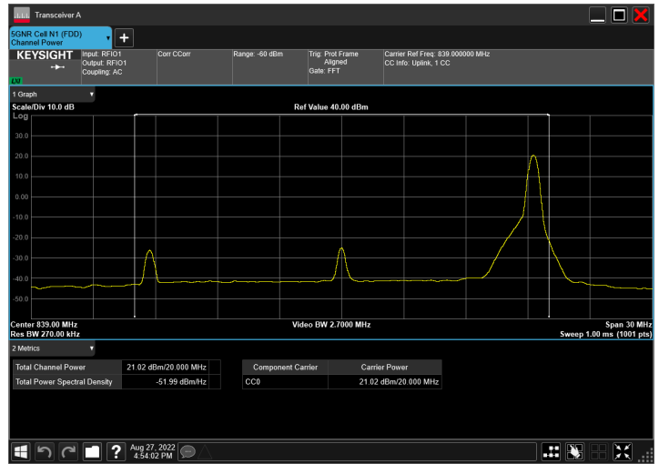
n5_20MHz_15kHz_839MHz_CP-OFDM 16 QAM_RB106@0
