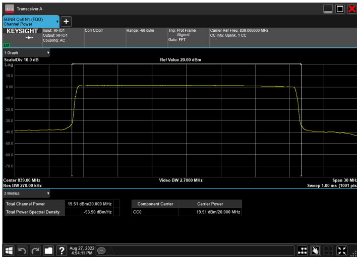
n5_20MHz_15kHz_839MHz_CP-OFDM 64 QAM_RB106@0
