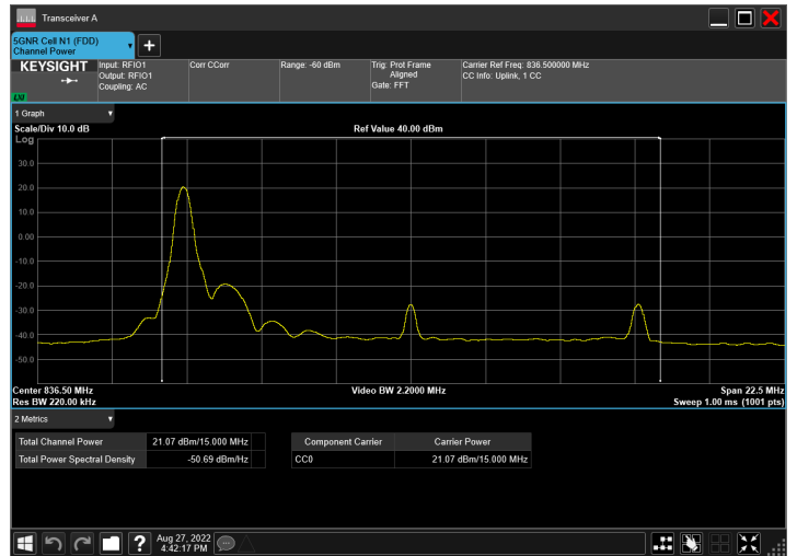
n5_15MHz_15kHz_836.5MHz_CP-OFDM QPSK_RB1@1
