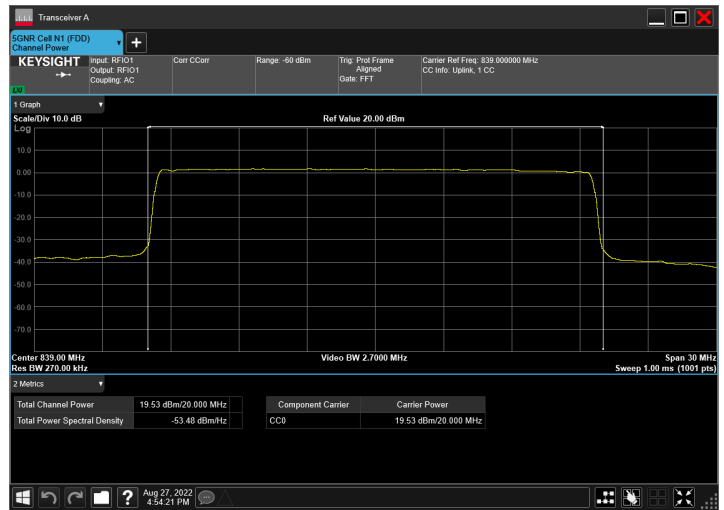
n5_20MHz_15kHz_839MHz_CP-OFDM 256 QAM_RB106@0
