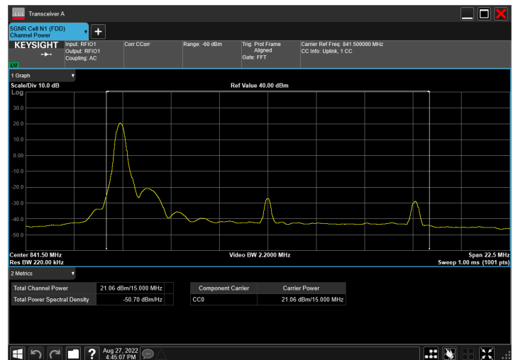
n5_15MHz_15kHz_841.5MHz_CP-OFDM QPSK_RB1@1
