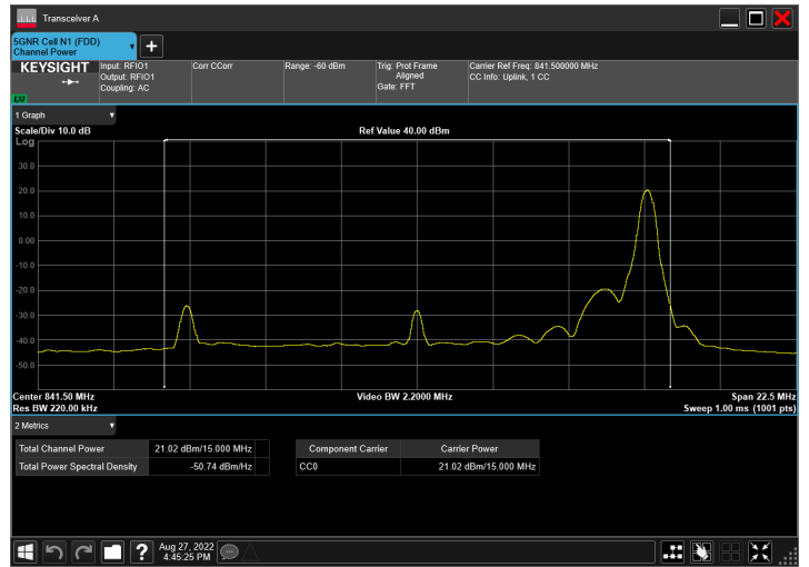
n5_15MHz_15kHz_841.5MHz_CP-OFDM 16 QAM_RB79@0
