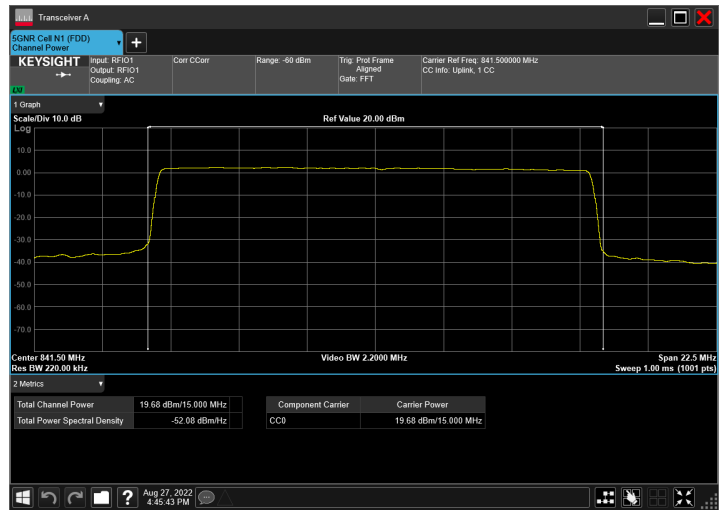
n5_15MHz_15kHz_841.5MHz_CP-OFDM 256 QAM_RB79@0
