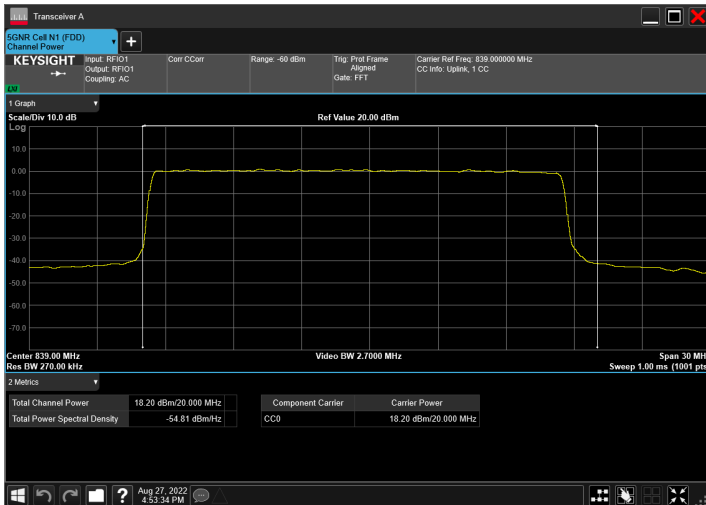
n5_20MHz_15kHz_839MHz_DFT-s-OFDM 256 QAM_RB100@0
