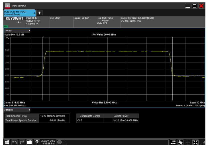
n5_20MHz_15kHz_834MHz_CP-OFDM 256 QAM_RB106@0
