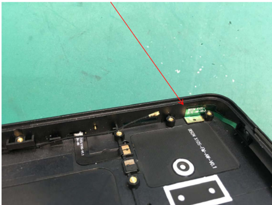
Aux antenna (Support PCS1900, WCDMA B2, LTE B2, LTE B41)
