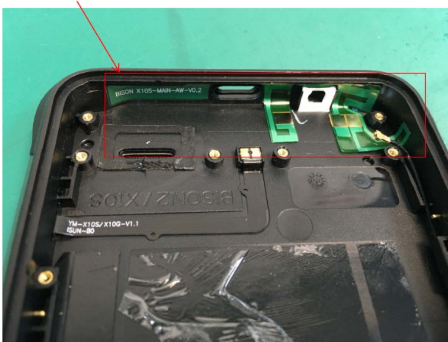
Aux antenna (Support PCS1900, WCDMA B2, LTE B2, LTE B41)
