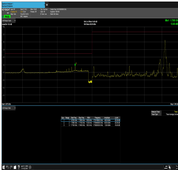
n66_30MHz_15kHz_1725MHz_DFT-s-OFDM QPSK_RB1@159
