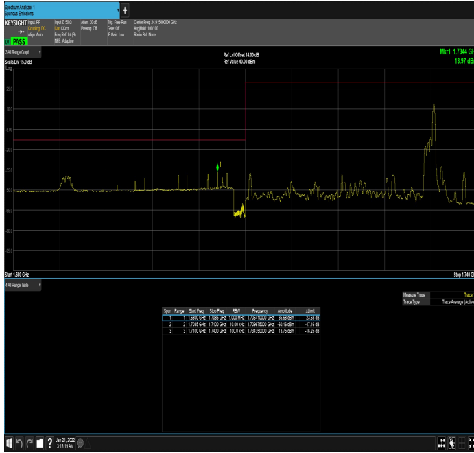
n66_25MHz_15kHz_1722.5MHz_DFT-s-OFDM QPSK_RB1@132
