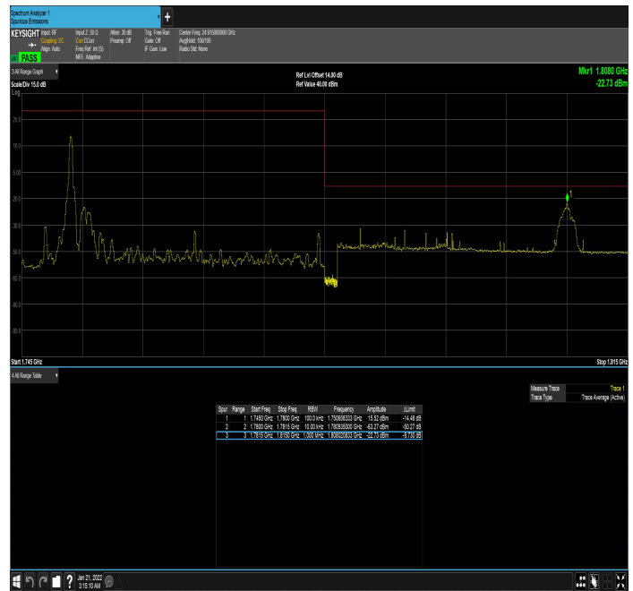
n66_30MHz_15kHz_1765MHz_DFT-s-OFDM QPSK_RB1@0
