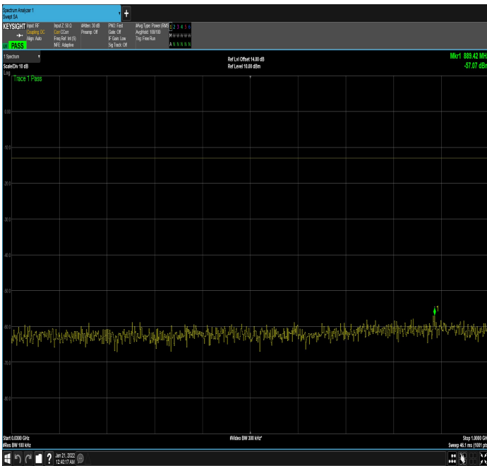
n66_40MHz_15kHz_1730MHz_DFT-s-OFDM QPSK_RB1@215|30MHz_1GHz
