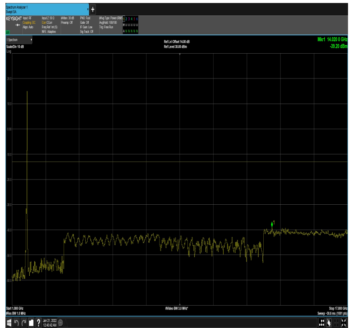
n66_40MHz_15kHz_1730MHz_DFT-s-OFDM QPSK_RB1@215|1GHz_17.80GHz
