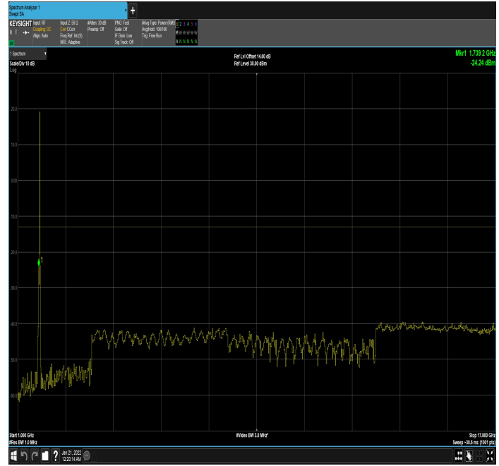
n66_20MHz_15kHz_1770MHz_DFT-s-OFDM QPSK_RB1@105|1GHz_17.80GHz
