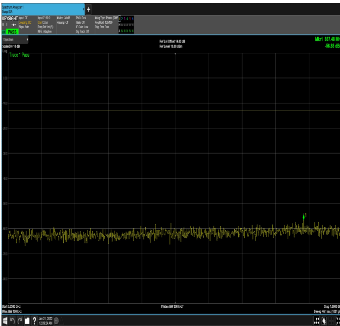
n66_15MHz_15kHz_1745MHz_DFT-s-OFDM QPSK_RB75@0|30MHz_1GHz
