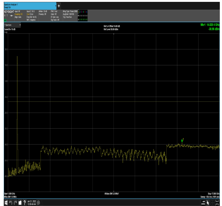
n66_15MHz_15kHz_1745MHz_DFT-s-OFDM QPSK_RB75@0|1GHz_17.80GHz
