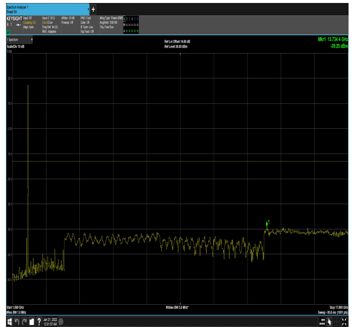
n66_10MHz_15kHz_1775MHz_DFT-s-OFDM QPSK_RB1@0|1GHz_17.80GHz
