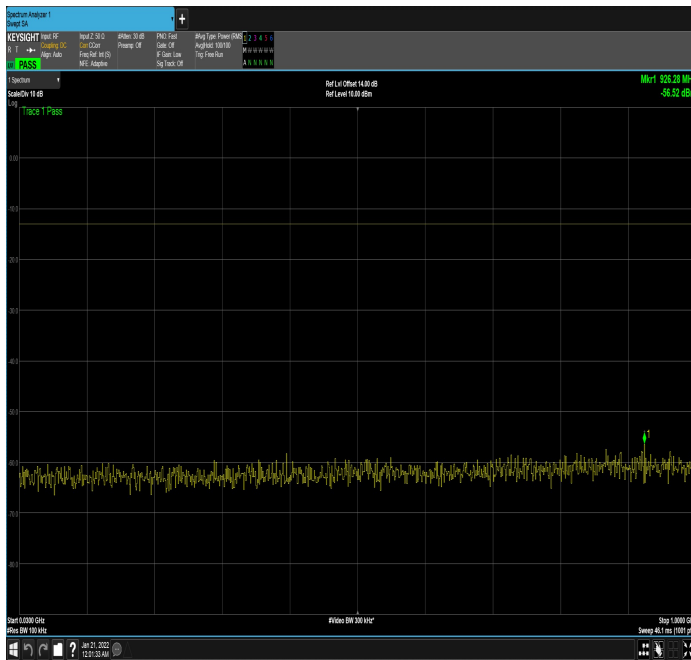
n66_10MHz_15kHz_1775MHz_DFT-s-OFDM QPSK_RB1@0|30MHz_1GHz
