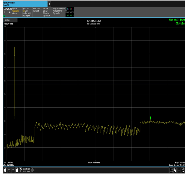
n66_10MHz_15kHz_1745MHz_DFT-s-OFDM QPSK_RB50@0|1GHz_17.80GHz
