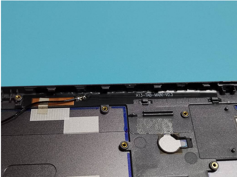
2/3/4G ANT
