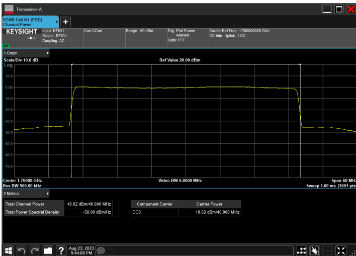
n66_40MHz_15kHz_1760MHz_CP-OFDM 64 QAM_RB216@0
