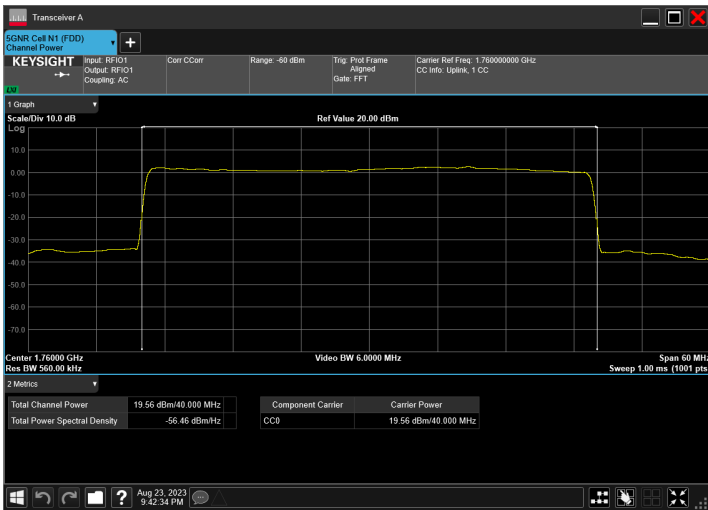
n66_40MHz_15kHz_1760MHz_DFT-s-OFDM 16 QAM_RB216@0
