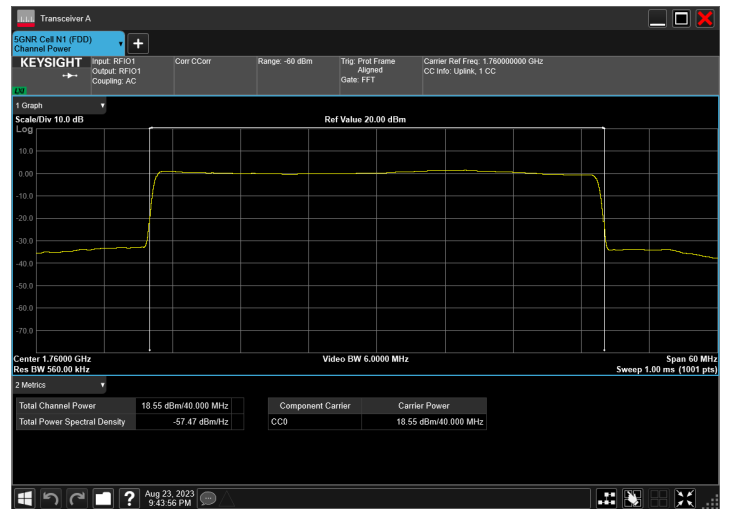
n66_40MHz_15kHz_1760MHz_CP-OFDM 16 QAM_RB216@0
