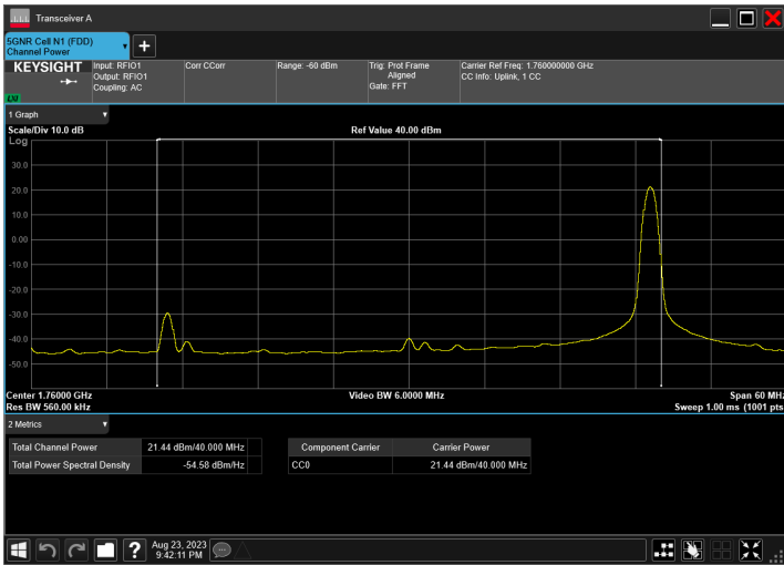
n66_40MHz_15kHz_1760MHz_DFT-s-OFDM QPSK_RB1@214
