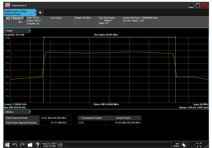
n66_40MHz_15kHz_1760MHz_CP-OFDM 256 QAM_RB216@0
