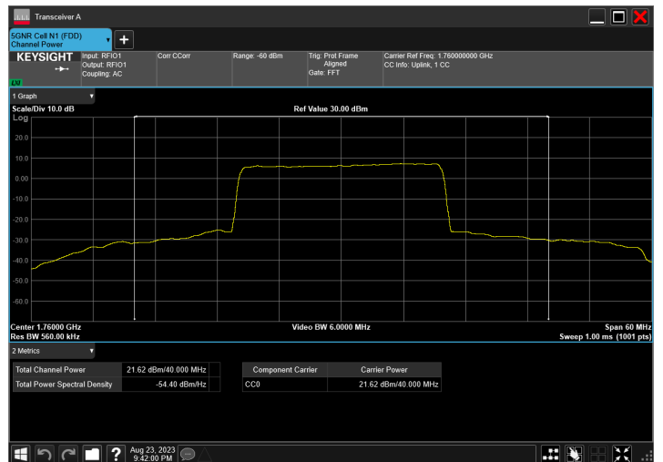
n66_40MHz_15kHz_1760MHz_DFT-s-OFDM QPSK_RB108@54
