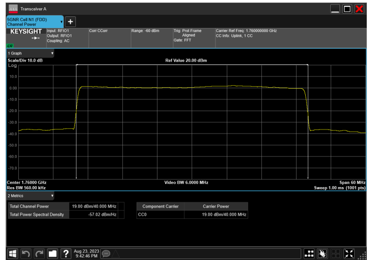
n66_40MHz_15kHz_1760MHz_DFT-s-OFDM 64 QAM_RB216@0
