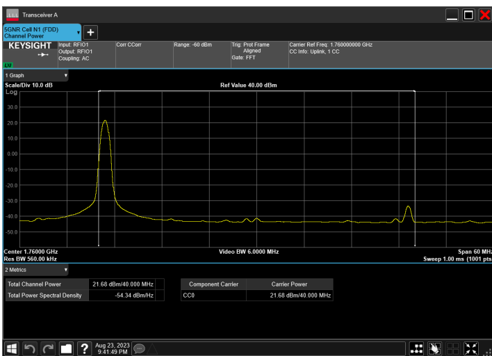
n66_40MHz_15kHz_1760MHz_DFT-s-OFDM QPSK_RB1@1
