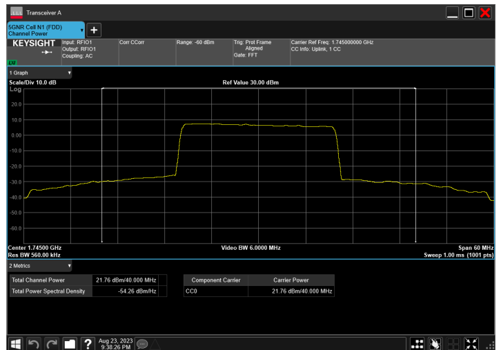
n66_40MHz_15kHz_1745MHz_DFT-s-OFDM QPSK_RB108@54
