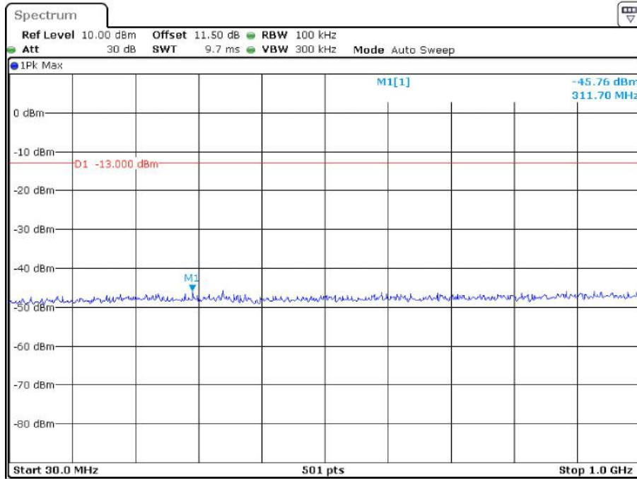
Band-2_1.4-MHz_Low_QPSK_RB6#0_1(30MHz-1GHz)
