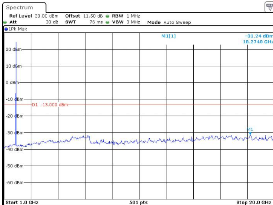
Band-2_1.4-MHz_Low_QPSK_RB6#0_2(1GHz-20GHz)
