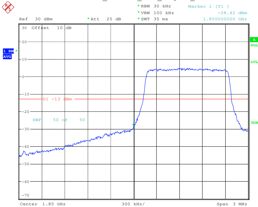
Band 2_1.4 MHz_Low_16QAM_RB6#0
