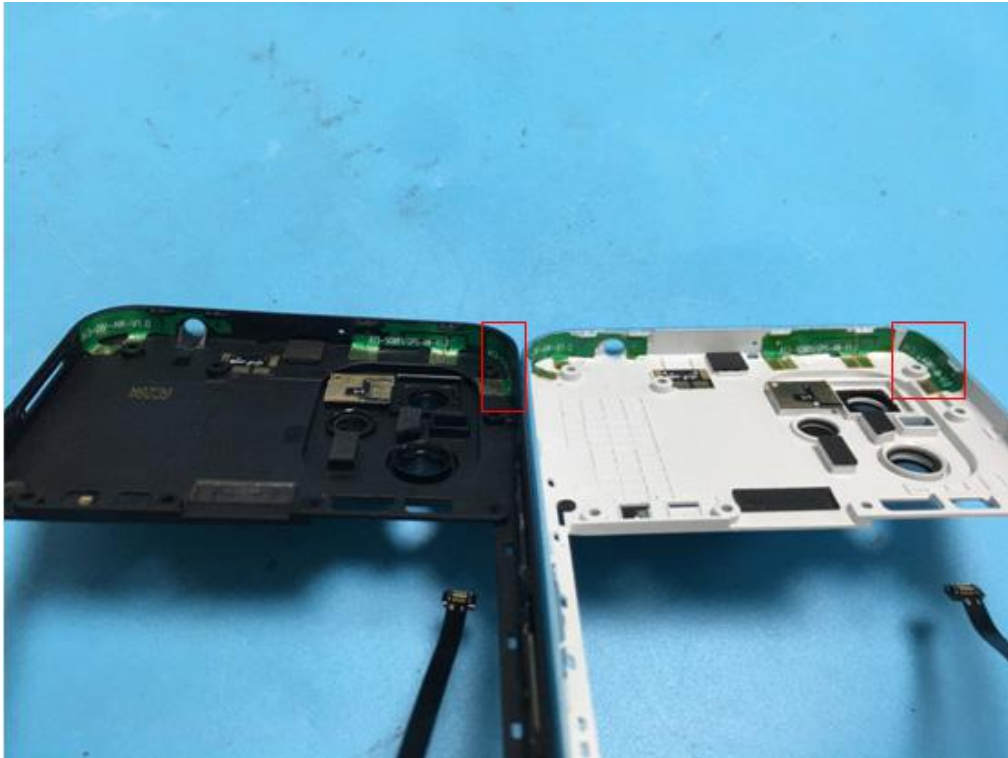
WWAN Aux Antenna
