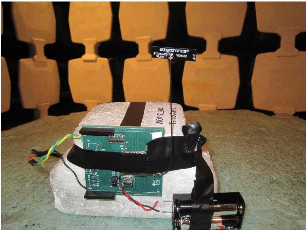
External Antenna – Horizontal Orientation
