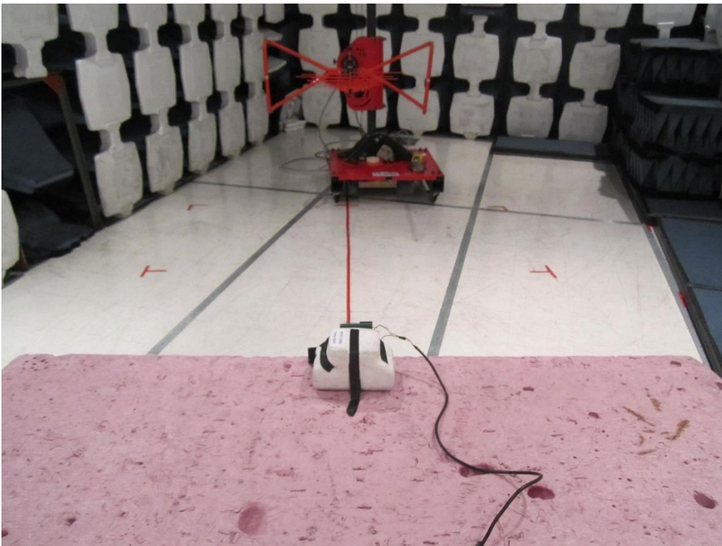
30MHz-1GHz Rear
