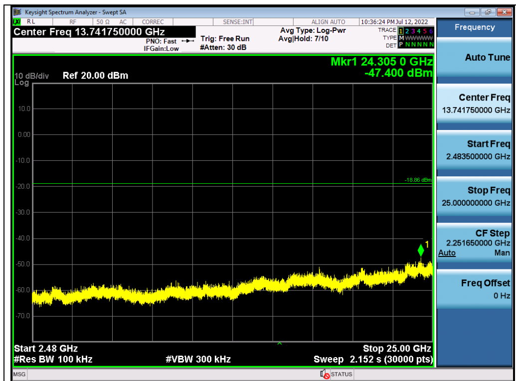
Test_Graph_GFSK_ANT1_2420_Higher Band Emissions
