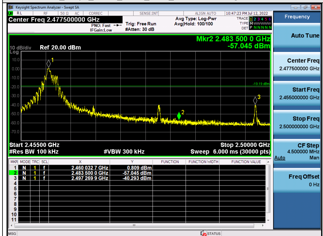
Test_Graph_GFSK_ANT1_2460_Higher Band Edge Emissions
