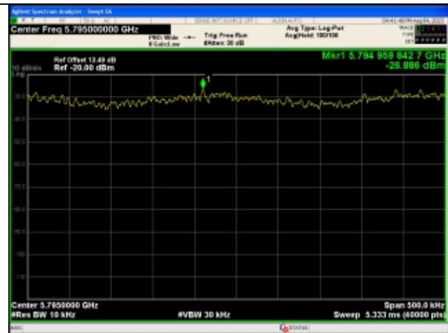
NT/NV_Antenna 0 IEEE 802.11n_Channel 159_40MHz
