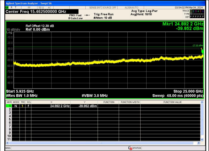
Spurious Emission:5925~25000.0 MHz IEEE 802.11ac Channel 149 20MHz Antenna 0
