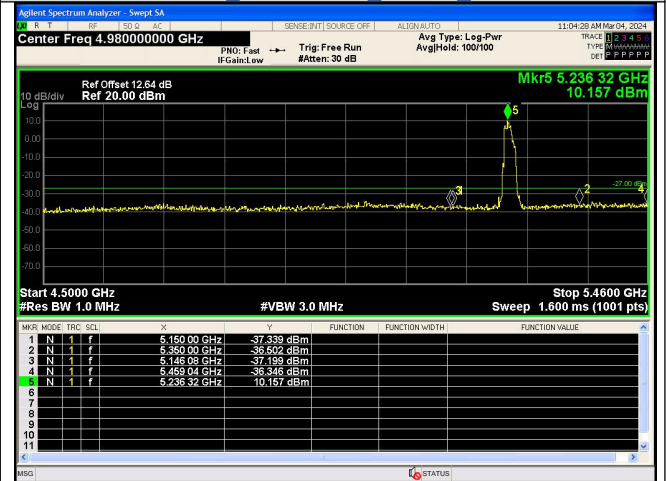
Out Of Band Emission IEEE 802.11n Channel 48 20MHz Antenna 0
