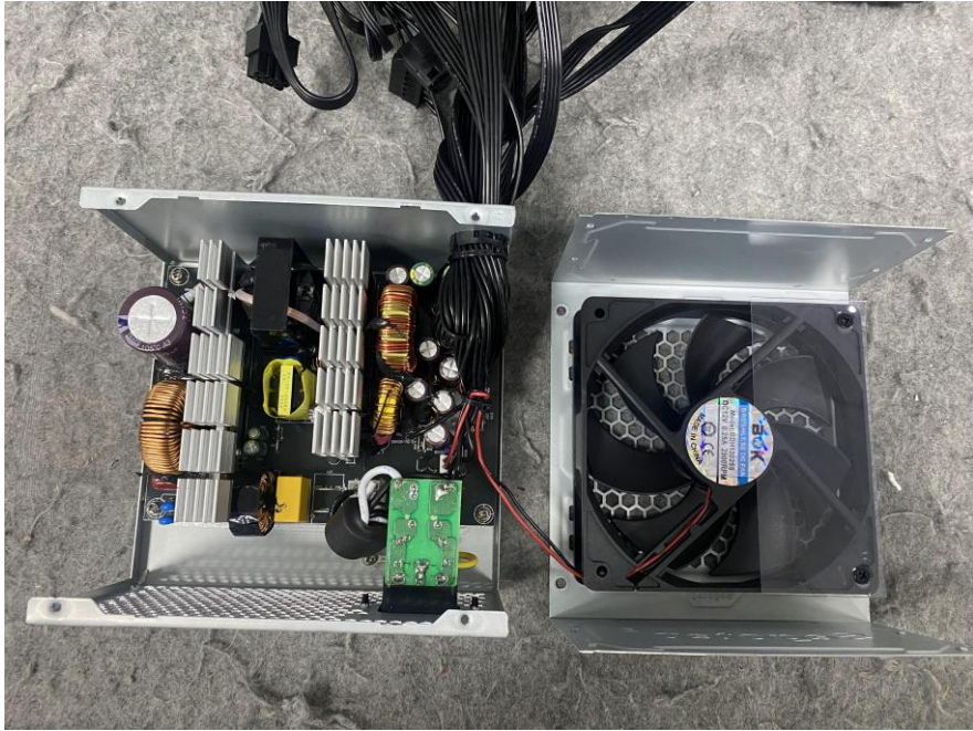
EUT View
