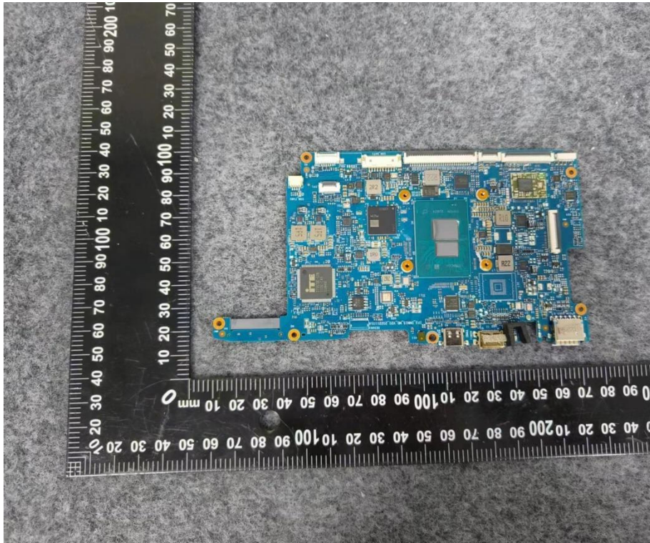
EUT View
