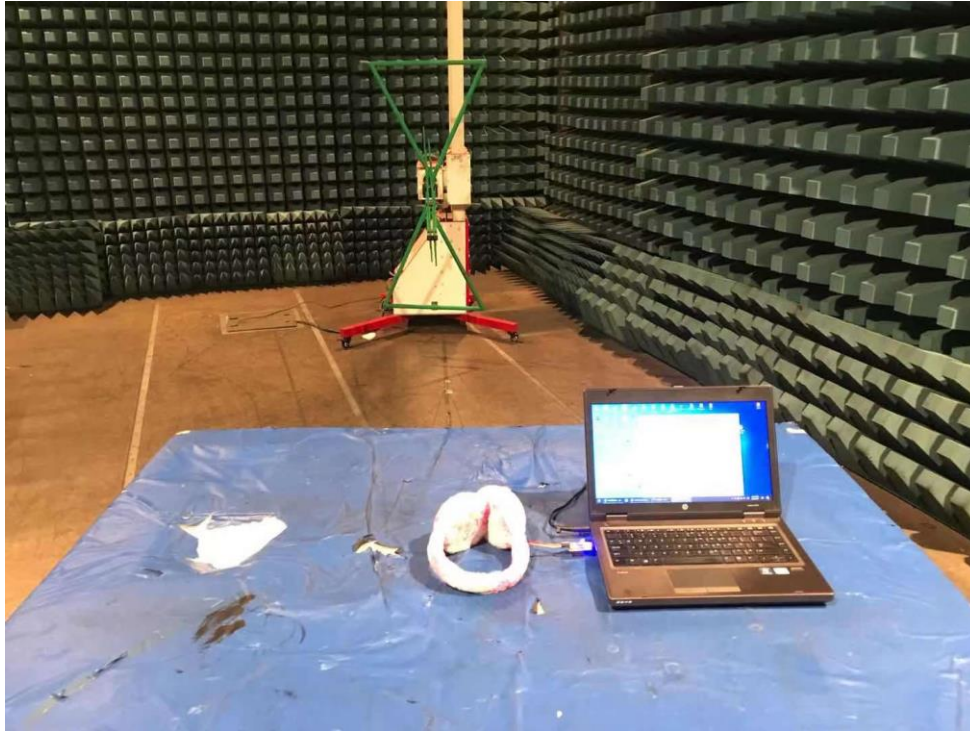
Below 1GHz
