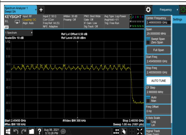
8DPSK,Hopping,3DH5,2454.5~2483.5MHz
