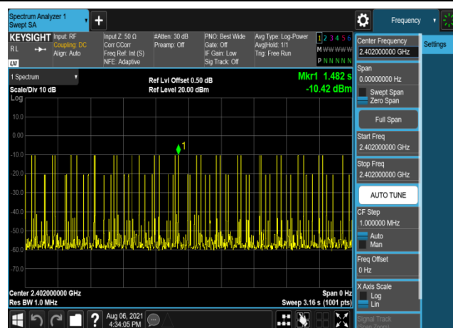
GFSK,2402,DH3,Transmission Number
