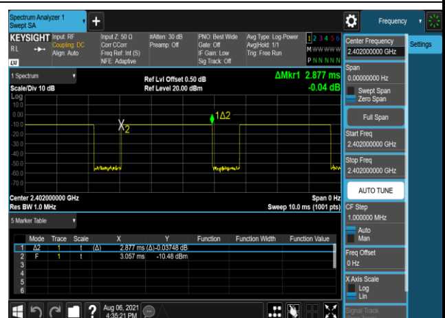
DQPSK,2402,2DH5,Transmission Time
