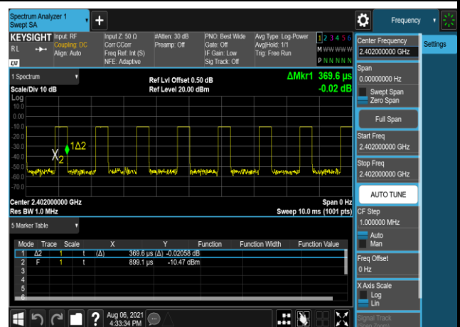
GFSK,2402,DH3,Transmission Time
