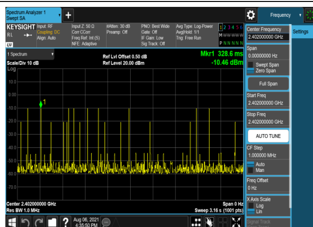
DQPSK,2402,2DH5,Transmission Number
