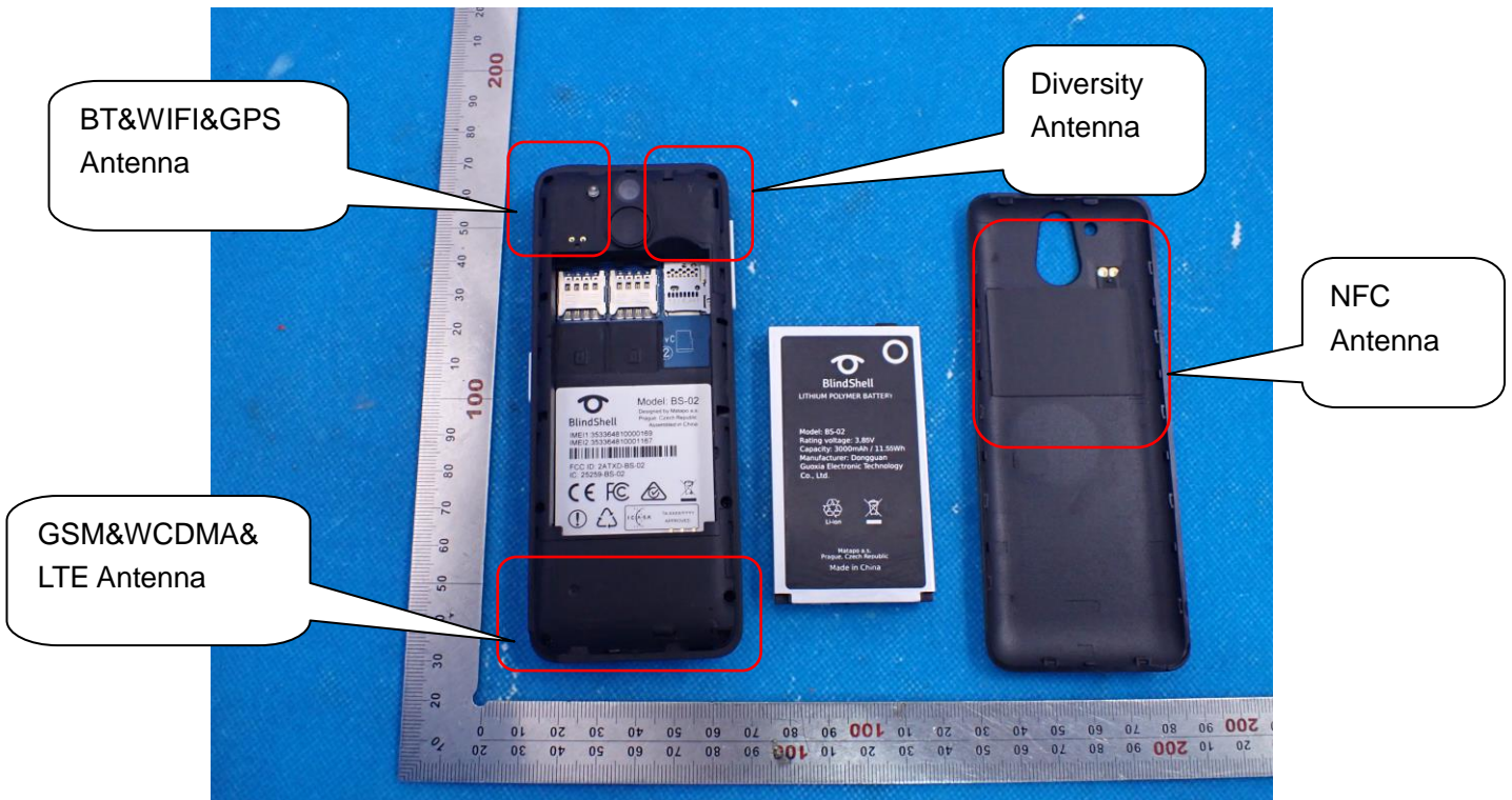
OPEN VIEW OF EUT(FIGURE 2)
