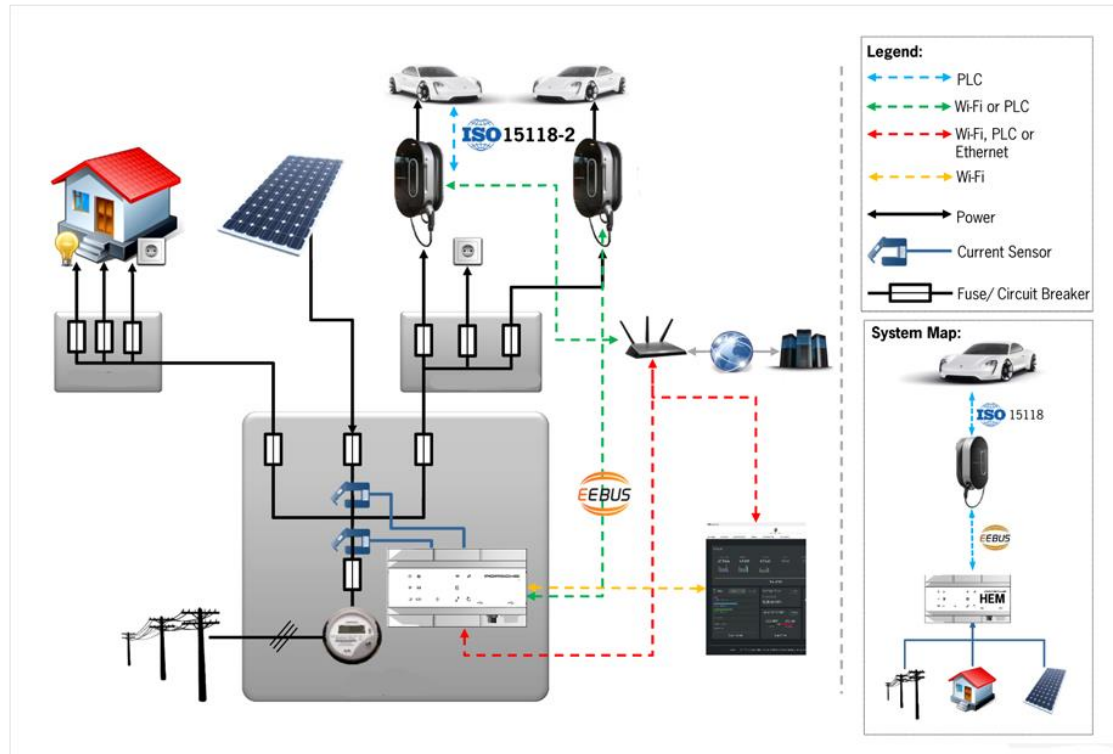
Fig. 1: Integration of the Home Energy Manager
