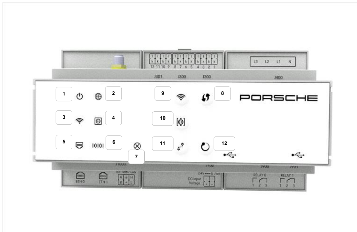
Fig. 2: Home Energy Manager displays and controls
