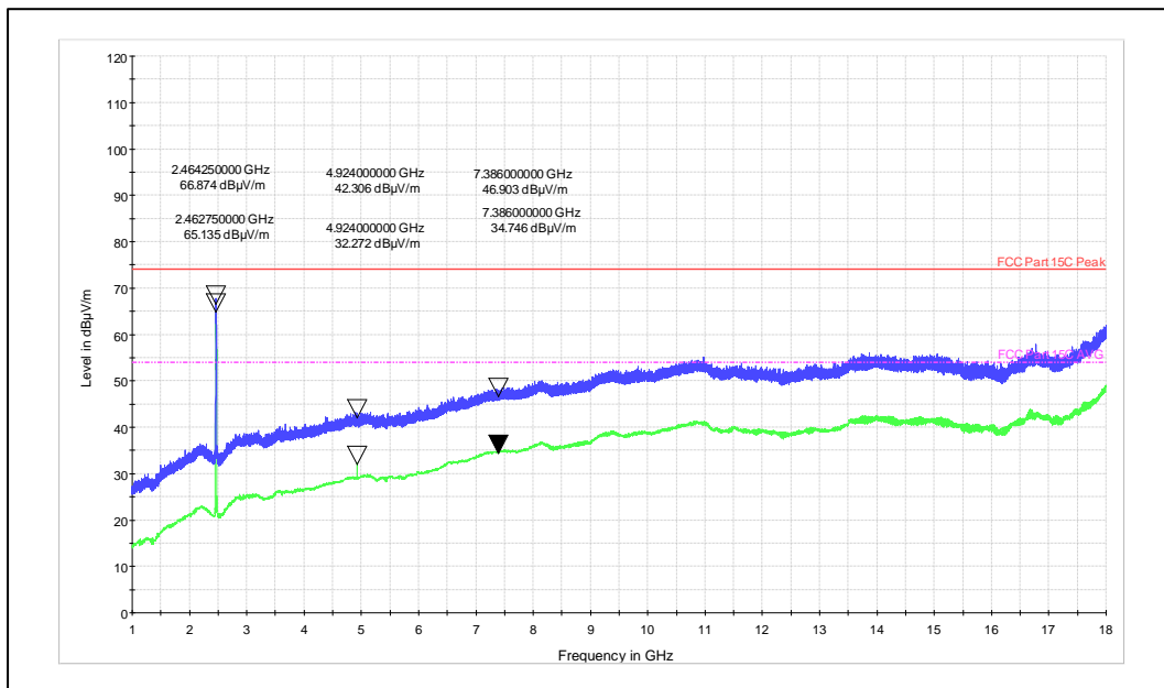
Channel Frequency: 1GHz – 18 GHz
