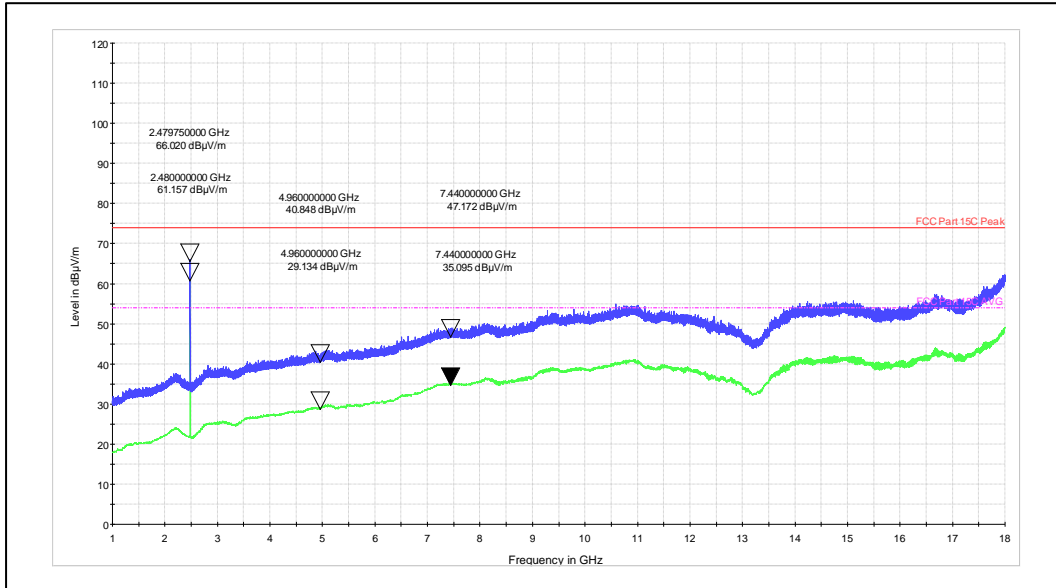
Channel Frequency: 1 GHz– 18 GHz
