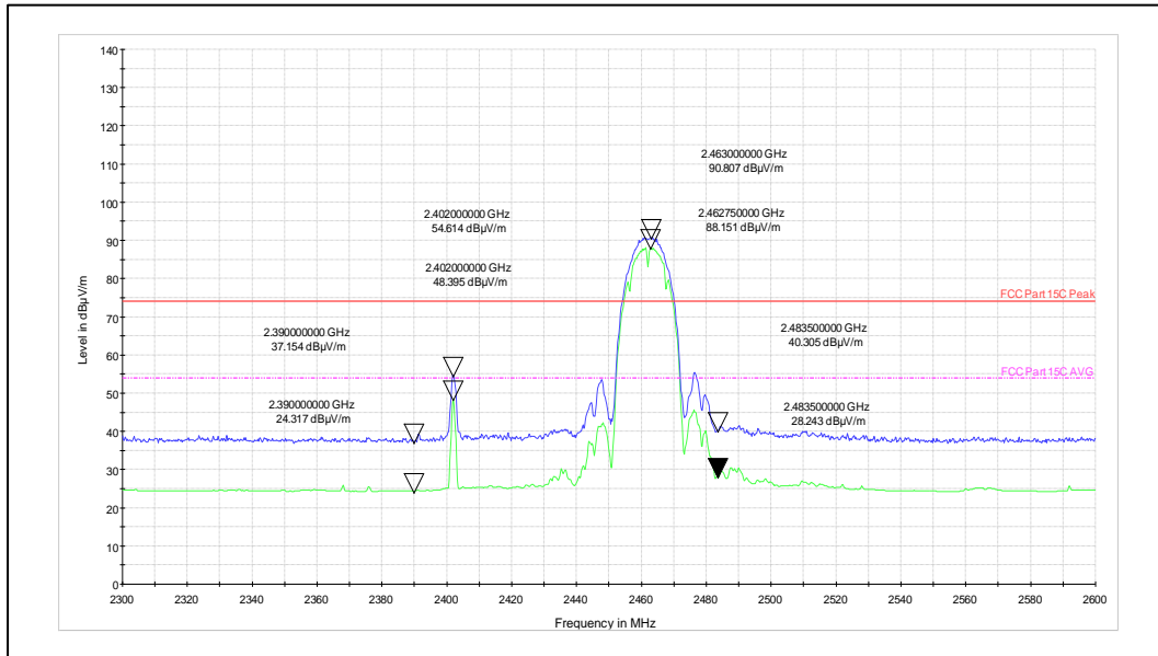
Channel Frequency: 2402MHz and 2462MHz
