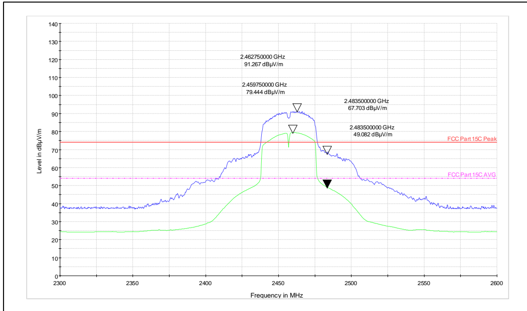
Channel Frequency: 2457MHz
