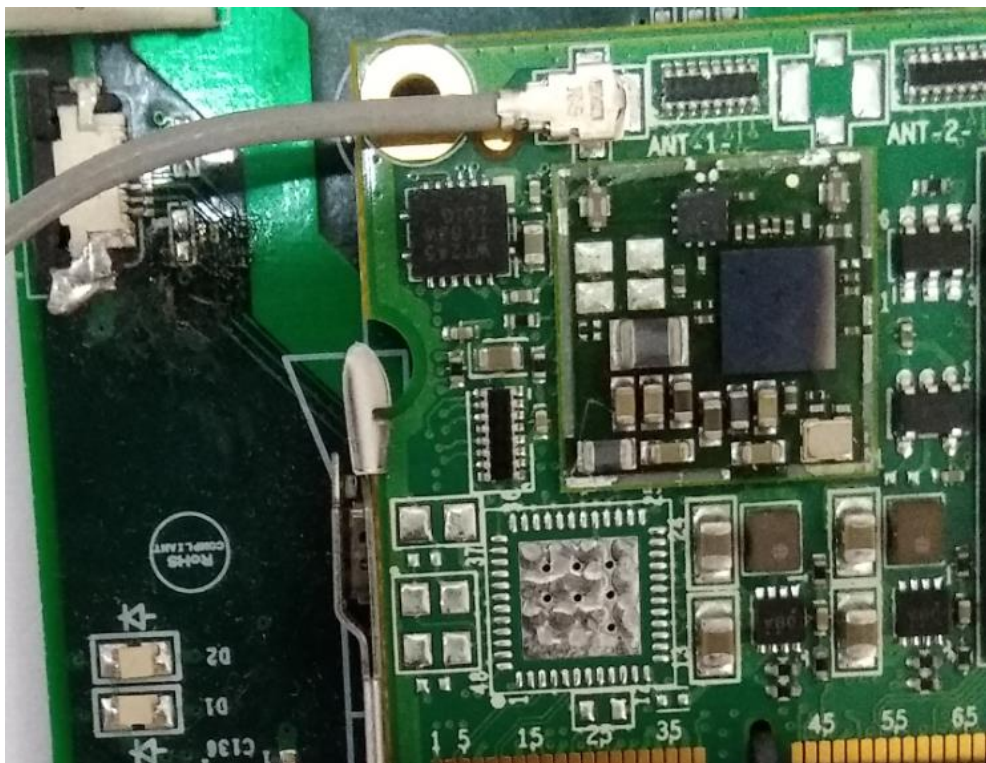
Photo 2: Antenna Part View
