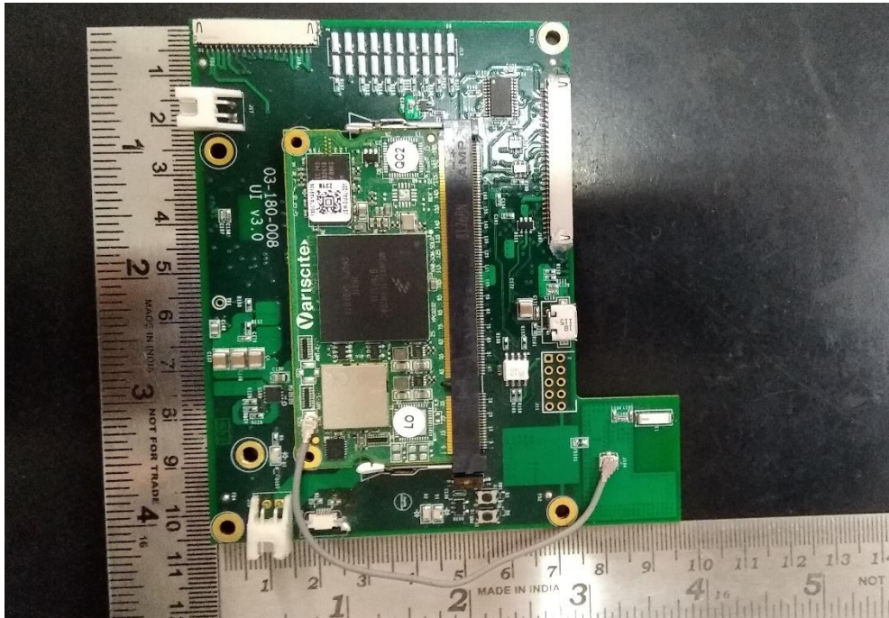
Photo 1: EUT Internal PCB dimensional view
