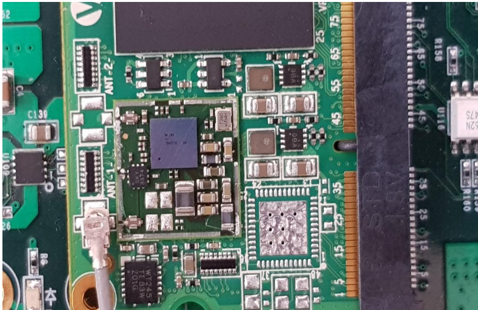
Photo 5: Radio Part with removed Enclosure
